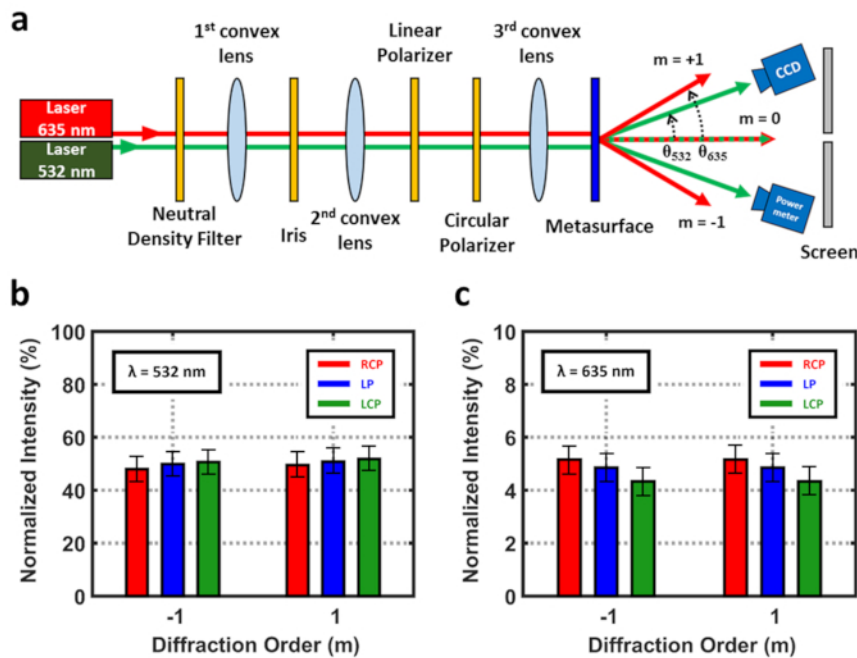
Figure 1: Diffracted beam power measurement. (a) The optical setup for the laser illumination. The next two panels show the measured diffracted beam power (b) at \lambda = 532 nm and (c) at 635 nm. Since the laser beam power was not consistent, the measured beam powers are calculated by time-averaging recorded values. The error bars in the figure represent the maximum and minimum values during the recording time. This figure has been modified from Yoon et al. 10 . Please click here to view a larger version of this figure.
