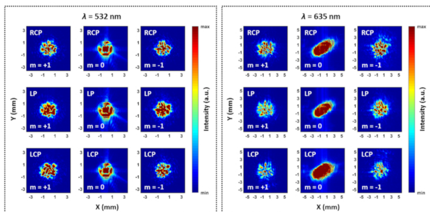
Figure 3: Captured beam profiles by CCD taken 14 cm behind the metasurface. The beam diameters can be estimated at \sim 3 mm at \lambda = 532 nm and \sim 5 mm at \lambda = 635 nm. The corresponding beam diverging angles are approximately 2.5^\circ and 4.1^\circ , respectively. The captured beam profiles have laser speckles, but they can be removed by diffusers 1 or Damman grating 3,15 . This figure has been modified from Yoon et al. 10 . Please click here to view a larger version of this figure.
