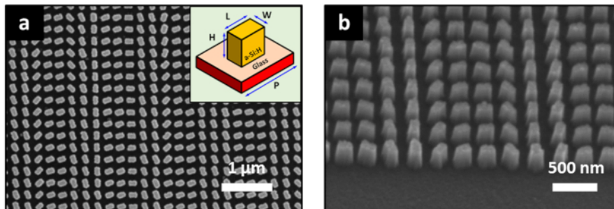
Figure 2: SEM images of the fabricated metasurface. (a) Top view of the metasurface. (inset) Geometry of the unit cell: length (L) = 150 nm, width (W) = 80 nm, height (H) = 300 nm, and pitch (P) = 240 nm. (b) Perspective view of the metasurface. This figure has been modified from Yoon et al. 10 . Please click here to view a larger version of this figure.
