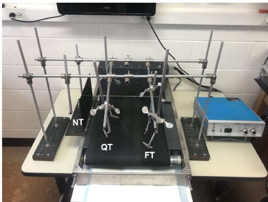
Figure 2: Training station setup. Body weight support mechanism surrounding the treadmill for either NT (far left), QT (middle), or FT (right) groups. Please click here to view a larger version of this figure.
