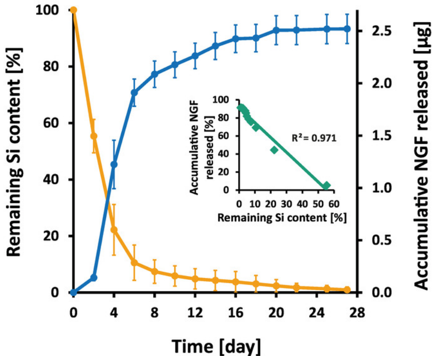
Figure 2: NGF release and Si erosion profiles of NGF-loaded PSiO 2 carriers. The extent of degradation of the PSiO 2 carriers is presented as the fraction of the remaining Si content at each time point out of the total Si content of the porous film. The inset shows the correlation between the accumulative NGF released and remaining Si content. Error bars represent SD, n=3. Please click here to view a larger version of this figure.
