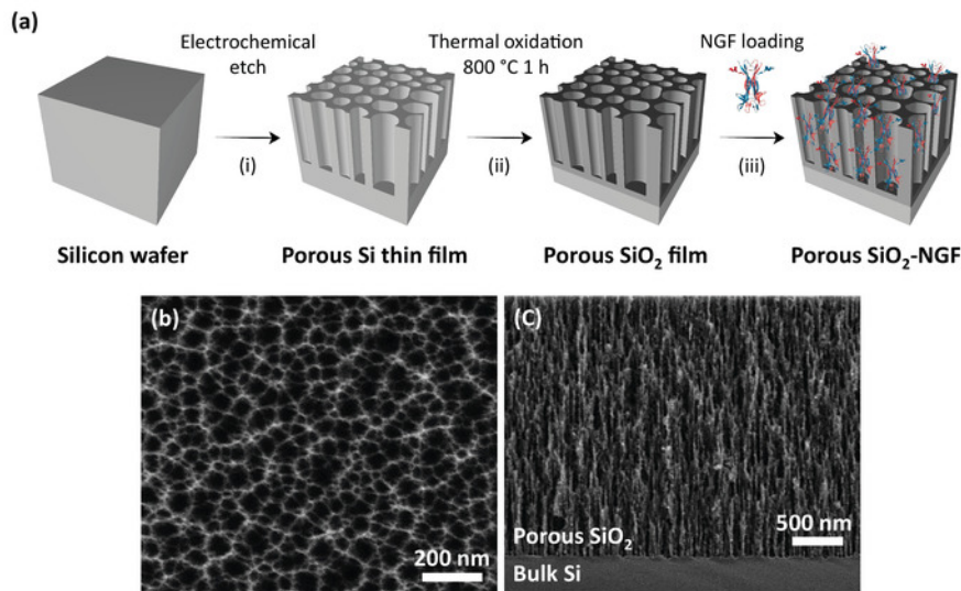
Figure 1: Fabrication of PSiO 2 films. (a) Fabrication scheme of the PSiO 2 carriers: (i) Silicon wafer is subjected to electrochemical etching for 20 s at 250 mA/cm 2 , followed by (ii) thermal oxidation at 800 °C to produce a PSiO 2 scaffold, and (iii) NGF loading by physical adsorption (schematics are not drawn to scale). (b-c) Top-view and cross-section electron micrographs of a characteristic PSiO 2 film. Please click here to view a larger version of this figure.
