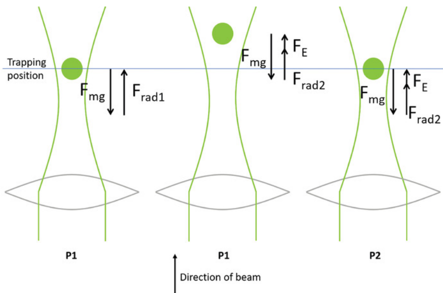
Figure 7: Determination of droplets charge. A schematic sketch of the procedure to determine the absolute charge of an optically levitated droplet. Please click here to view a larger version of this figure.
