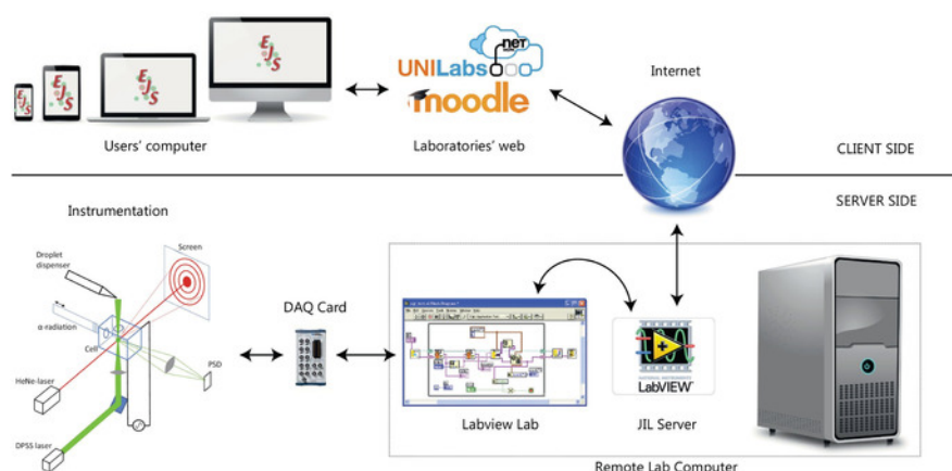
Figure 1: Architecture of the remote laboratory experimentation. Internet users connect to the UNILabs webpage using their computer or mobile devices. The web environment serves the remote lab JavaScript application that allows to remotely operate the experiment. This application connects to a computer located in the laboratory through the JIL server middleware, which enables the communication between JavaScript applications and LabVIEW programs. Finally, the lab computer communicates with the experimental setup using the necessary DAQ cards and a LabVIEW program. Please click here to view a larger version of this figure.
