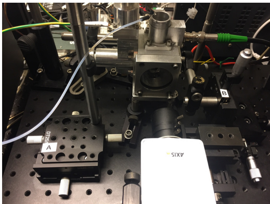
Figure 4: Detail of the experimental setup. The droplet dispenser is shown at the top of the image, the cell in the middle and, at the bottom, the web camera. Letter A: the translation stage used to adjust the position of the dispenser inside the cell. Letter B: The lens used by the PSD to perceive the trapped droplet. Please click here to view a larger version of this figure.
