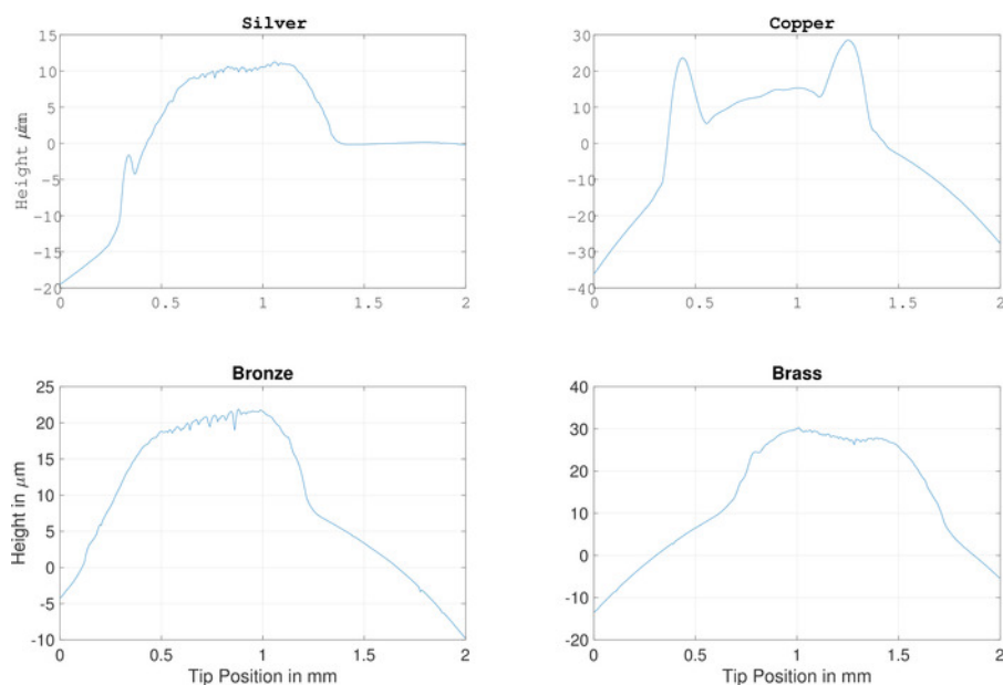
Figure 6: Height profiles for the conductive tracks on the insulator for metal substrates, determined using the profilometer. This figure has been modified from Faller et al. 39 . Please click here to view a larger version of this figure.
