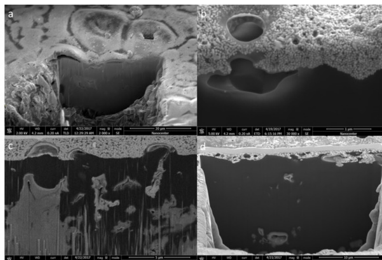
Figure 8: FIB images of conductive ink on the insulator and metallic substrates. These images show (a) copper, (b) bronze, (c) titanium, and (d) brass. This figure has been modified from Faller et al. 39 . Please click here to view a larger version of this figure.
