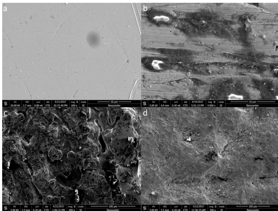
Figure 1: SEM images of the metallic substrates. These images show (a) copper, (b) bronze, (c) steel, and (d) titanium. They are taken at different magnifications as illustrated by the scale bar in the lower right corner of each image. Based on these images, the surface homogeneity can be assessed. This figure has been modified from Faller et al. 39 . Please click here to view a larger version of this figure.
