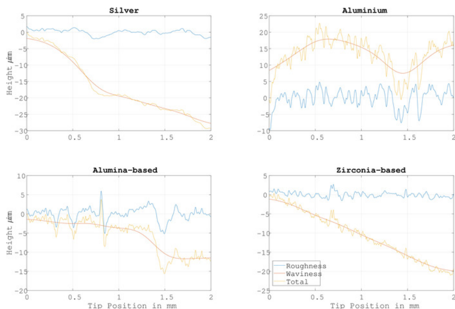
Figure 2: Profilometer measurements of metallic and ceramic AM substrates. The roughness values R_a and R_q in nanometers are determined according to ISO 4287. For silver, the values are 689.39 nm and 788.06 nm, respectively; for aluminum, they are 2151.19 nm and 2750.38 nm, respectively; for alumina-based ( Al_2O_3 ) substrates, they are 1210.47 nm and 1737.6 nm, respectively; for zirconia-based ( ZrO_2 ) substrates, they are 559.97 nm and 681.56 nm. The waviness is the more widely spaced surface texture of the substrate. The waviness is the remaining texture in-homogeneity with the roughness component removed. This figure has been modified from Faller et al. 39 . Please click here to view a larger version of this figure.
