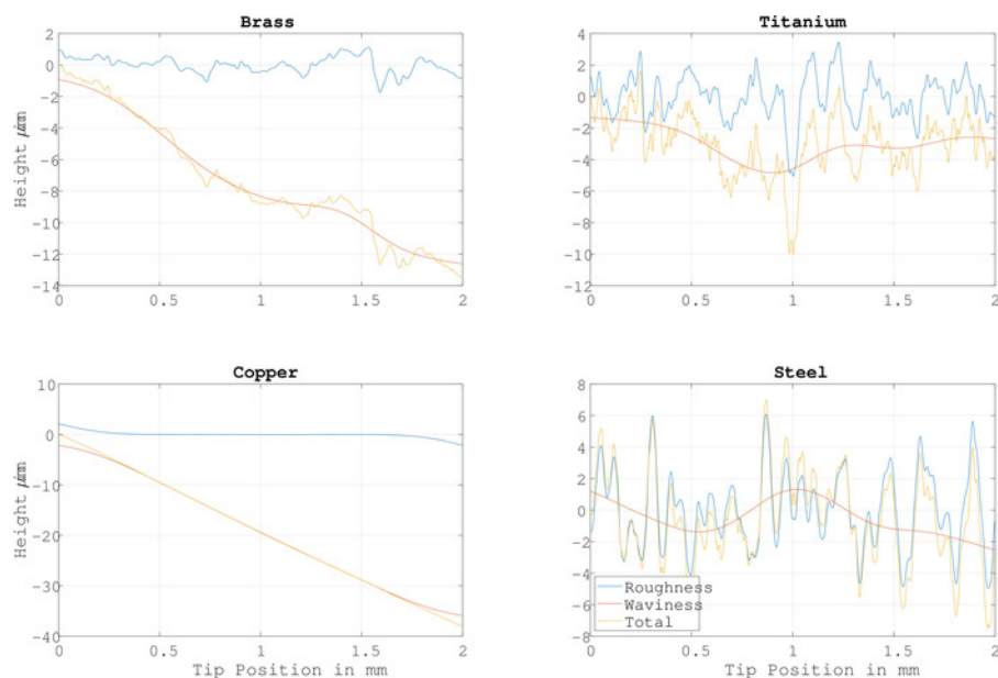
Figure 3: Profilometer measurements of metallic substrates. The R_a and R_q values for the respective substrates are, for brass, 414.2 nm and 494.49 nm, respectively; for titanium, 1099.86 nm and 1448.06 nm, respectively; for copper, 307.63 nm and 358.92 nm, respectively; for steel, 1966.95 nm and 2238.78 nm, respectively. This figure has been modified from Faller et al. 39 . Please click here to view a larger version of this figure.
