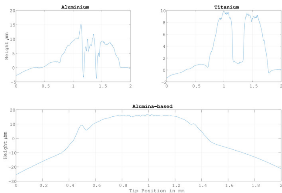
Figure 7: Height profiles for the conductive tracks on metal and ceramic substrates, determined using the profilometer. This figure has been modified from Faller et al. 39 . Please click here to view a larger version of this figure.
