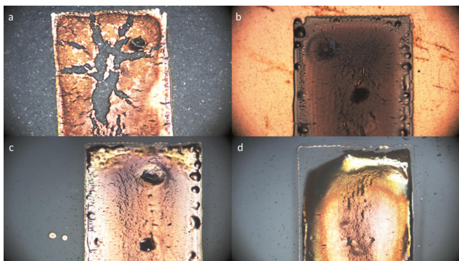
Figure 5: Microscopic images of conductive ink printed onto an insulator and an AM metal substrate after photonic curing. The substrates are (a) aluminum, (b) copper, (c) \text{Al}_2\text{O}_3 , and (d) \text{ZrO}_2 . The width of the conductive structure in each image is w = 1 mm. The integrity of the conductive structure on aluminum is completely destroyed, whereas the structures on copper and \text{Al}_2\text{O}_3 remain intact. This figure has been modified from Faller et al. 39 . Please click here to view a larger version of this figure.
