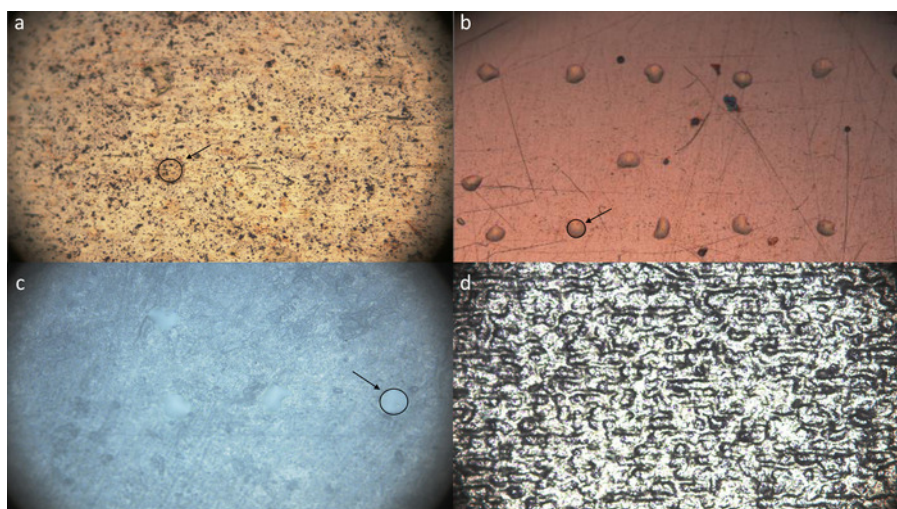
Figure 4: Drop size tests for metallic and ceramic substrates. These images show (a) bronze, (b) copper, (c) \text{ZrO}_2 , and (d) steel. Distinct drops measured here are marked (where possible) by arrows in the respective image. The determined drop sizes are gathered in Table 3 . This figure has been modified from Faller et al. 39 . Please click here to view a larger version of this figure.
