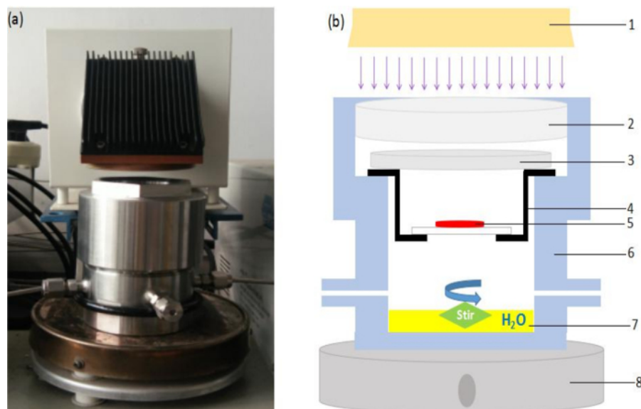
Figure 1: Concentrating light reactor system for the photocatalytic reduction of \text{CO}_2 . (A) Photograph of the set-up. (B) Schematic of the set-up. 1 = Xe lamp, 2 = quartz glass window, 3 = Fresnel lens, 4 = holder, 5 = photocatalyst, 6 = stainless steel reactor, 7 = \text{H}_2\text{O} , and 8 = magnetic stirrer. Please click here to view a larger version of this figure.
