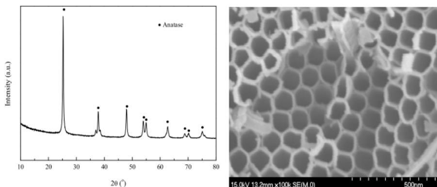
Figure 2: X-ray diffraction (XRD, left) and scanning electron microscope (SEM, right) of \text{TiO}_2 by anodization. Please click here to view a larger version of this figure.
