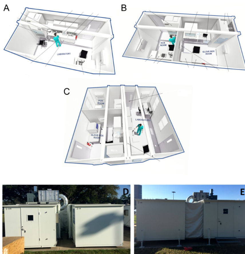
Figure 2: Schematics. (A) The basic laboratory BSL-2. (B) The BSL-3 module includes the glove box and PCR laboratories, which have a common pass-through window for protected specimen transfer. (C) Connected laboratory facilities (A) and (B) with shared utilities. (D, E) Photographs of the connected units from opposite sides. Please click here to view a larger version of this figure.
