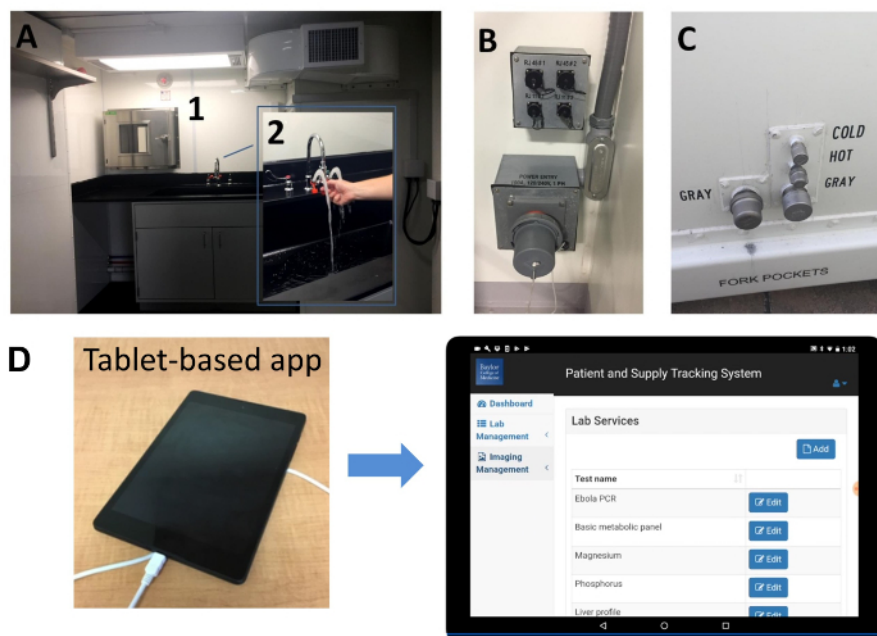
Figure 3: Schematics. A. Interior of the BSL-3 facility has a pass-through window (1), a sink and eyewash station (2) at inlet. B. Electrical power connectors. C. Water connectors. D. Tablet-based software for supply tracking and laboratory result documentations. Please click here to view a larger version of this figure.
