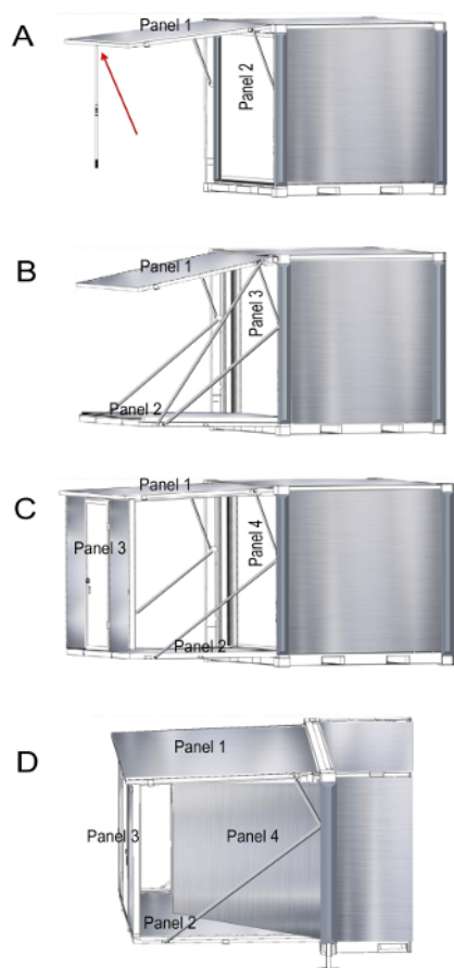
Figure 4: Deployment of the laboratory facility. Instruction for panels unfolding on one side of the unit as illustrated (A-D). Please click here to view a larger version of this figure.
