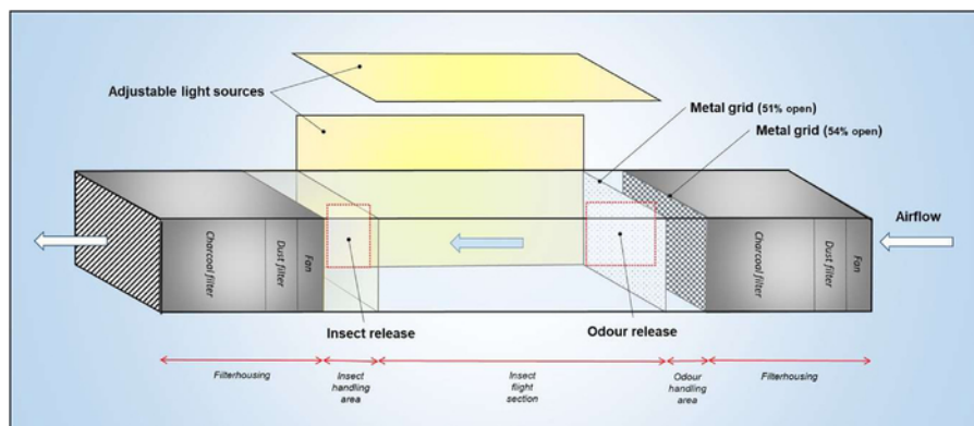
Figure 1. Schematic of wind tunnel located as NIBIO, Ås - Norway. The wind tunnel is placed in a climate controlled room. The airflow is filtered by activated charcoal filters before and after odor application, and is then circulated back into the room. Please click here to view a larger version of this figure.
