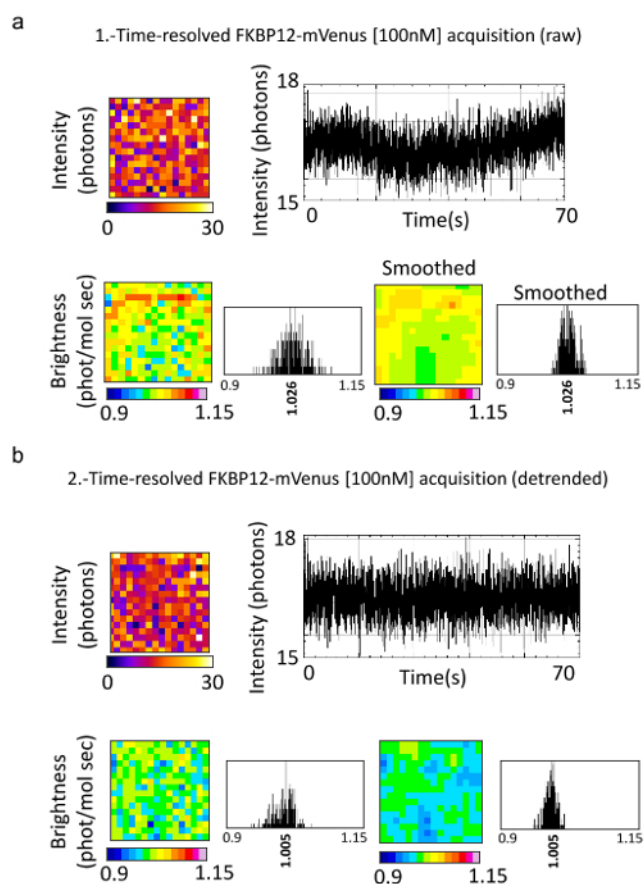
Figure 2. Automatic detrending is needed to accurately measure a population of monomers in solution. (a) A stack of 5000 16 x 16 pixel images was acquired as described in Protocol section. The intensity of the first frame is shown together with the average time-resolved intensity profile, which shows long term fluctuations that might be related to bleaching and other solvent and/or photophysics effects. Whatever the cause for these long-term fluctuations, they impact the brightness calculations and hence require detrending. Without automatic detrend, one gets B = 1.026 , whereas after automatic detrending, B = 1.005 . Also, the brightness without (left panels, second row) and with (right panels, second row) smooth filtering is shown. (b) The same data presented in (a) was detrended and the results in terms of intensity and brightness shown. Please click here to view a larger version of this figure.
