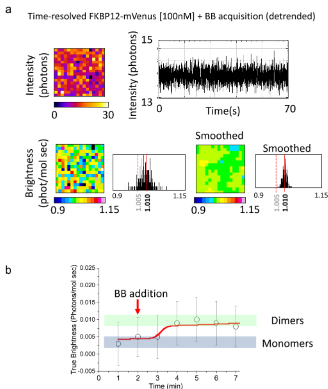
Figure 3. In-vitro N&B is able to resolve the transition between FKBP12F36V monomers and dimers in real time. The addition of the dimerizer drug BB resulted in a two-fold increase in true brightness right after 2 min (from 0.005 to 0.010 in true molecular brightness). (a) The intensity of the first frame is shown together with the mean intensity profile of the detrended image. The brightness without (left panels, second row) and with (right panels, second row) smooth filtering is shown. (b) Mean brightness is plotted (every 5000 frames) using the true molecular brightness \epsilon . The dimerization occurs 2 minutes after BB addition ( t = 1 min) at t = 4 min. The fitted curve is a sigmoidal function to stress the tendency toward dimerization after addition of the dimerizer drug (BB). Error bars represent the standard error of the brightness distribution at each time point. Please click here to view a larger version of this figure.
