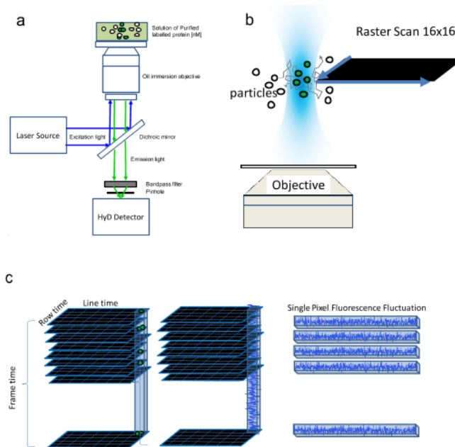
Figure 1. Application of N&B to detect protein monomer-dimer transitions in solution. (a) Simplified optical path of a laser scanning microscope (LSM) equipped with a laser source (set at 514 nm in the case of mVenus labeled proteins) directed (blue arrows) toward an immersion objective (in our case a 63X1.4NA oil) illuminating a 100 nM solution of FKBP12F36V-mVenus solution. The emission fluorescence (green arrows) passes through a dichroic mirror and is directed toward a bandpass filter that cleans the emission light, and a pinhole set at 1 Airy unit situated right before a point digital detector capable of photon counting. (b) A confocal volume of illumination is scanned through 16 x 16 pixels illuminating single FKBP12F36V-mVenus molecules that enter and exit the Gaussian shape confocal volume producing an array of fluorescence intensity fluctuations. (c) Image series acquired over time. Please click here to view a larger version of this figure.
