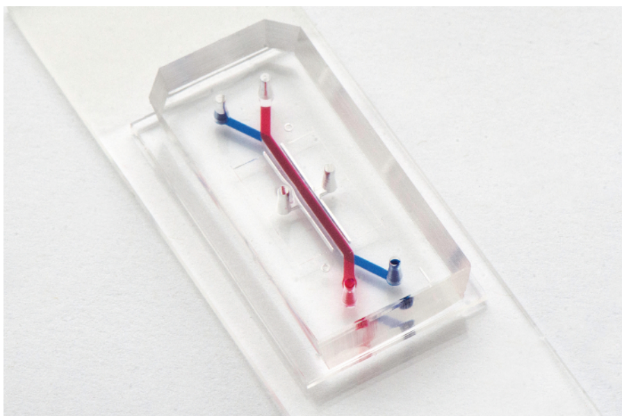
Figure 4: Photograph of an assembled PDMS Organ Chip. Red dye fills the larger apical channel used for parenchymal cells while the blue dye highlights the basal channel typically used for vascular endothelium. Please click here to view a larger version of this figure.
