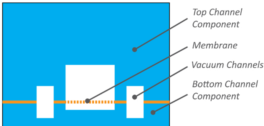
Figure 1: Organ Chip cross section. Organ Chips consist of two channels separated by a porous, elastic membrane that can be seeded with cells on both sides. Top channel cross sections are 1 mm wide x 1 mm high, bottom channel cross sections are 1 mm wide x 0.2 mm high, and vacuum channels in both and bottom parts are 0.3 mm wide, 0.5 mm high, and spaced 0.3 mm from the fluidic channels. Please click here to view a larger version of this figure.
