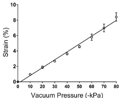
Figure 6: Application of membrane strain using vacuum side channels. Plot indicates linear strain modulation of membrane in response to an applied vacuum pressure. Cyclic uniaxial strain is applied uniformly to the culture region of the Organ Chip using applied vacuum to parallel side channels. The Strain correlates linearly with decreasing vacuum pressure at approximately 1% strain for every -10 kPa change in vacuum pressure ( R^2 = 0.992 ). Error bars indicate standard deviation of the mean. Please click here to view a larger version of this figure.
