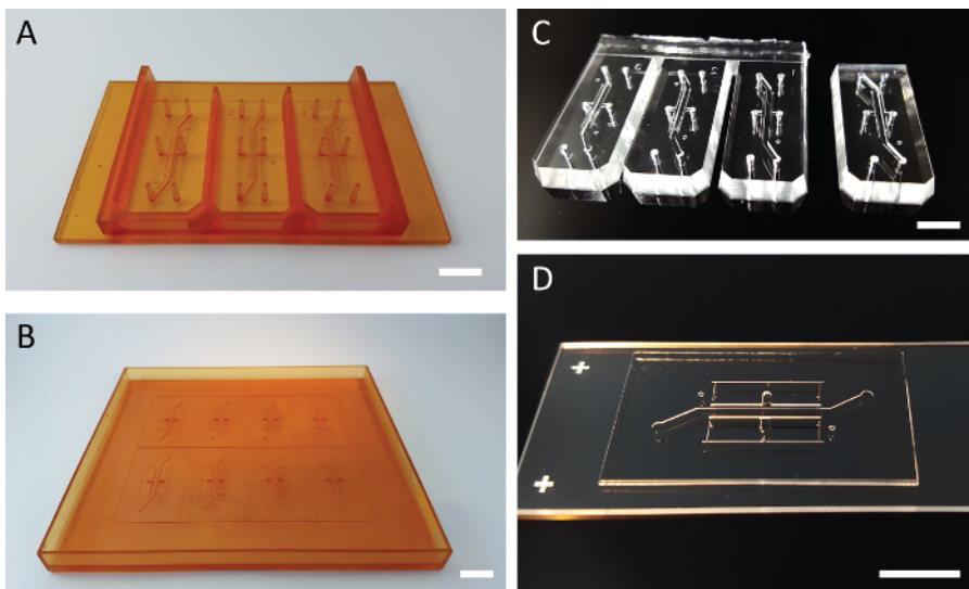
Figure 2: Channel fabrication with 3D printed molds. Organ chip parts are cast against high resolution 3D printed molds (A and B), which allows for greater design versatility and prototyping than traditional soft lithography. Top channel parts (C) are cured under compression eliminating the need for punching ports in the finished parts. Each triplicate casting is singulated with a single cut. Bottom channel parts (D) are placed on glass slides to facilitate ease of use and imaging. Scale bars are approximately 1 cm in all images. Please click here to view a larger version of this figure.
