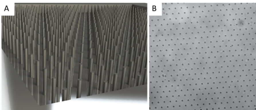
Figure 3: The porous PDMS membrane is cast using DRIE patterned silicon wafers. (A) Rendering of 7 \mu\text{m} diameter, 50 \mu\text{m} tall micropillars etched using DRIE into a silicon wafer. (B) PDMS is cured on this array under 4 kg of compression (16 kPa) to create a 50 \mu\text{m} thick membrane with an array of 7 \mu\text{m} diameter through holes spaced hexagonally 40 \mu\text{m} apart. Please click here to view a larger version of this figure.
