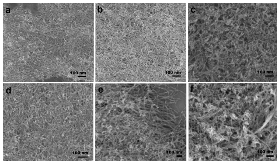
Figure 2: SEM images of the Au nanowires grown on substrate other than Si wafer. Nanowires grown from: (a) Al_2O_3 , (b) SrTiO_3 , (c) LaAlO_3 (d) glass slide, (e) ITO and (f) FTO substrates. Please click here to view a larger version of this figure.
