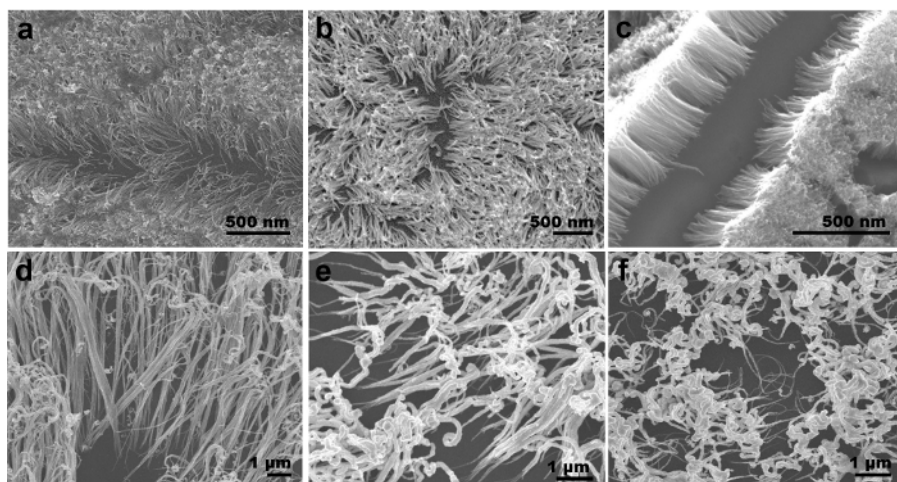
Figure 3: SEM images of the synthesized with other ligands. Ultrathin nanowire arrays formed with (a) MPAA, (b) 2-Naphthalenethiol, (c) 3-MBA ligands. Tapered Au nanowires formed with mixed ligands of 4-MBA and 3-MPA: (d) C_{4\text{-MBA}} : C_{3\text{-MPA}} = 3 : 1 , (e) C_{4\text{-MBA}} : C_{3\text{-MPA}} = 6 : 4 and (f) C_{4\text{-MBA}} : C_{3\text{-MPA}} = 1 : 1 . Please click here to view a larger version of this figure.
