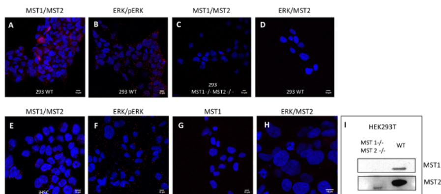
Figure 1: Representative PLA data. (A-H) Cells were fixed and stained with the indicated antibodies followed by the PLA procedure. Blue: DAPI, RED: PLA signal. Photomicrographs were obtained with a Leica SP5 confocal microscope. (I) Immunoblot for MST1 and MST2. Scale bar is 10 \mu m. Please click here to view a larger version of this figure.
