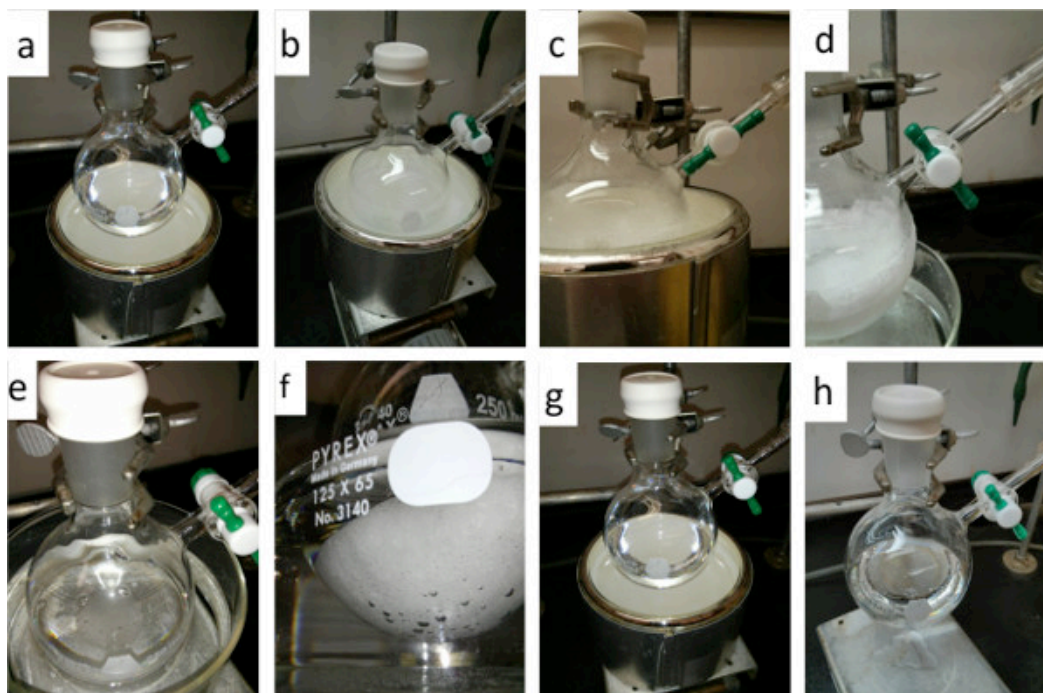
Figure 2. Detail photos of the freeze-pump-thaw steps: (a) step 1, place solvent in flask; (b) step 2, freeze the solvent in dry ice (or alternatively with liquid nitrogen); (c) step 3, introduce vacuum; (d) step 4, seal the flask under vacuum; (e), (f), step 5, thaw the solvent and observe evolution of gas bubbles; (g) step 7 repeat freeze thaw process (three cycles recommended); (h) step 8, seal the solvent under nitrogen.
