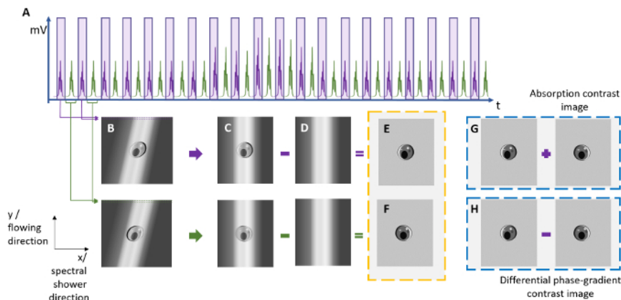
Figure 2: Reconstruction of ATOM Images from the Line-scan Time Trace. To reconstruct the ATOM images with the absorption contrast and differential (enhanced) phase-gradient contrast, two sets of time-stretched pulses (see the purple and green pulses) are extracted from (a) the time-multiplexed temporal waveform trace and are then digitally segmented and stacked to form (b) two 2D images showing the two opposite phase-gradient contrasts. Note that a shearing operation is needed to form (c) the distortion-free images by compensating for the sub-index shift due to the round-off error in the laser repetition rate estimation. By subtracting the (d) raw line-scan from the spectral intensity envelope of the laser source, the background of the images can be removed. (g) An absorption contrast image can be obtained by a pixel-by-pixel intensity summation of images (e) and (f), whereas (h) a differential phase-gradient contrast image can be obtained from the subtraction of images (e) and (f). Please click here to view a larger version of this figure.
