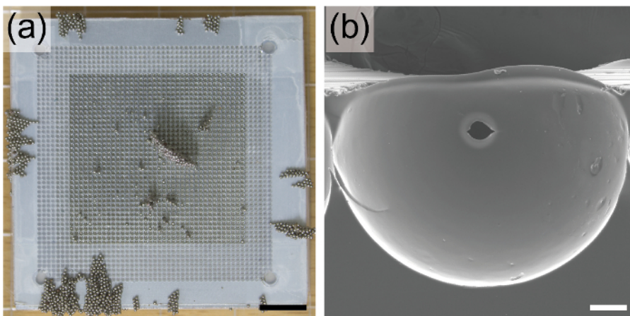
Figure 8: Limitation using single big magnet and of bead size. (a) Unlike the case of using an array of small magnets, when one large magnet is used, almost all of the beads tend to move to the edge or center of the magnet where the high density magnetic field is formed. Further, the beads are connected to form a chain shape. The scale bar is 10 mm. (b) SEM image of linked microwell which was fabricated by using \Phi 800\ \mu\text{m} beads with 1\ \text{mm} \times 1\ \text{mm} \times 1\ \text{mm} magnet array. Using a bead that is too large in size relative to the size of the magnet can create a small hole in the wall between adjacent microwells. The scale bar is 100\ \mu\text{m} . Please click here to view a larger version of this figure.
