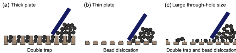
Figure 9: The importance of choosing the appropriate top plate thickness and hole size in the bead trapping process. (a) If the top plate is too thick, a double trap will occur. (b) Conversely, if the top plate is too thin, there is a tendency for the beads to come off. (c) If the size of the through-hole is larger than the bead diameter, both double trap and bead dislocation may occur. Please click here to view a larger version of this figure.
