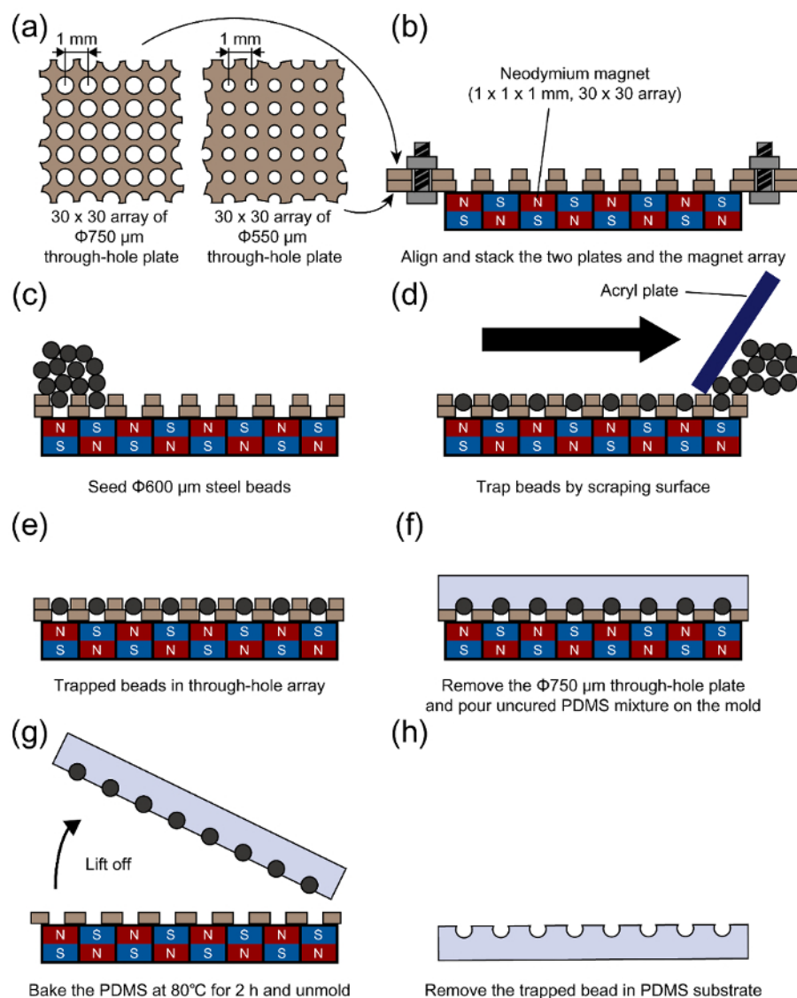
Figure 1: Schematic of fabrication process. (a) Making 30 x 30 \Phi 550 and 750 \mu\text{m} through-hole array in aluminum plates using CNC engraver. (b) Aligning the two through plates by using the alignment holes. Subsequently, the aligned plates were stacked on the magnet array. (c) Seeding a sufficient amount of steel beads onto the plates. (d) Scraping the beads using an acrylic plate to trap the beads in the through-hole array. (e) Beads were trapped in the through-hole array. (f) The top plate ( \Phi 750\text{-}\mu\text{m} through-hole array) was removed and uncured PDMS mixture was poured into the mold. (g) After the PDMS was baked at 80^\circ\text{C} for 2 h, the cured PDMS was unmolded. (h) The cured PDMS grabs the steel beads. The beads are then removed using a neodymium magnet ( \Phi 15 \text{ mm} with a thickness of 2 mm). Please click here to view a larger version of this figure.
