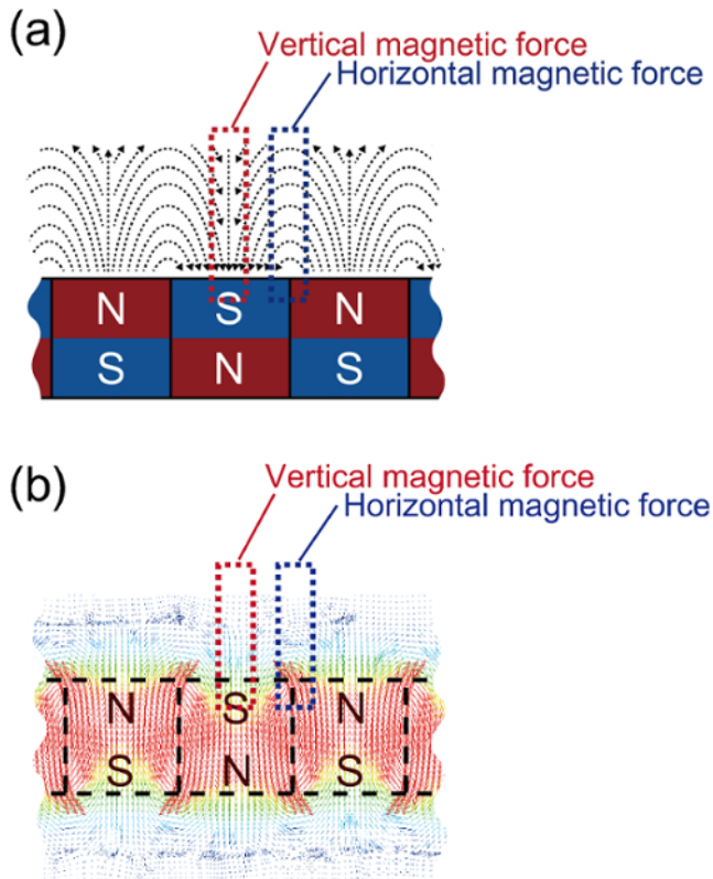
Figure 7: Magnetic field distribution of magnet array. Each magnet is of the opposite polarity to its neighbor. The horizontal magnetic field is dominant at the interface between neighboring magnets, while the vertical magnetic field is strongest at the center of each magnet. These directional forces guide a bead to the center of a magnet. (a) Magnetic field of magnet array. (b) Vector of magnetic field as determined by magnetostatic simulation. Please click here to view a larger version of this figure.
