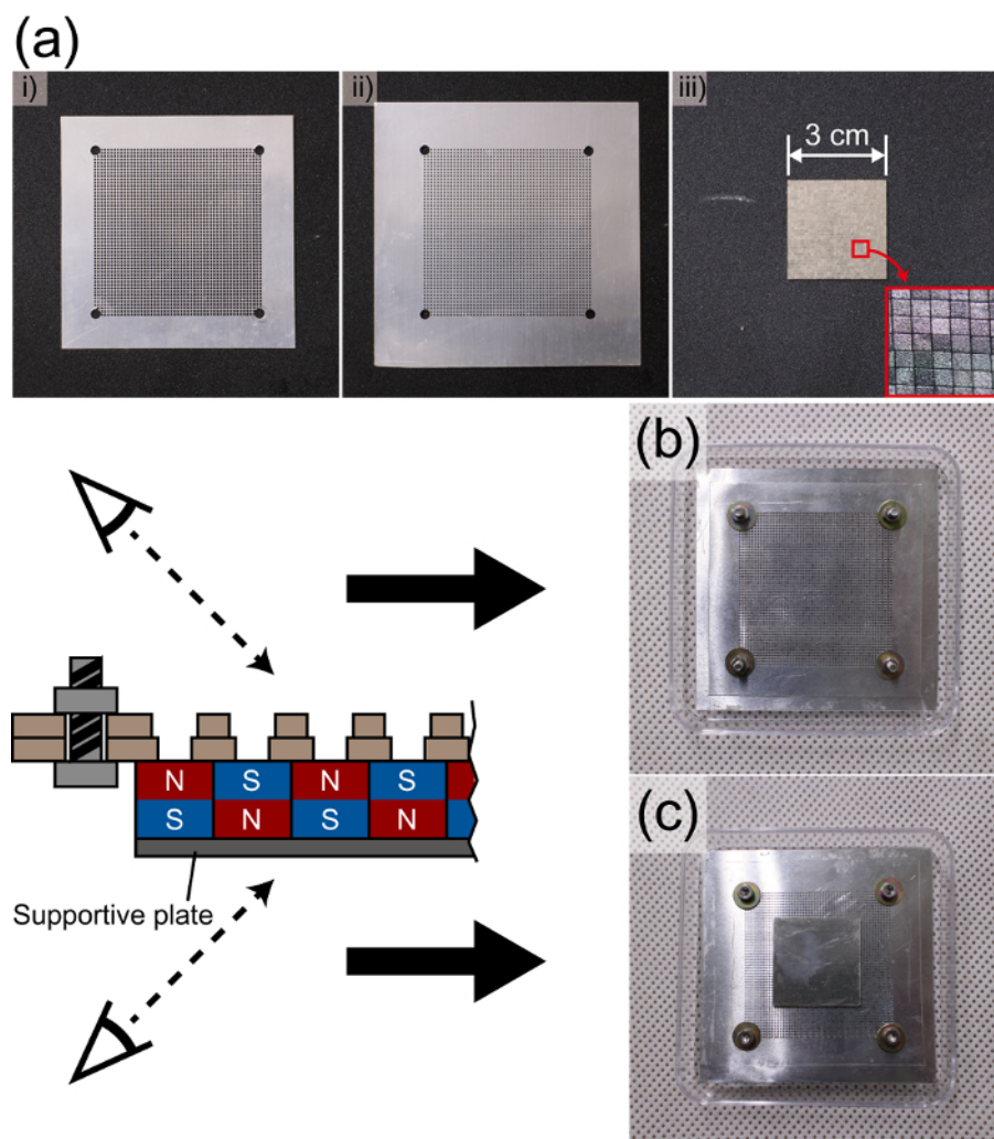
Figure 2: Fabrication process. (a) Preparing two through-hole plates and magnet array. i) Aluminum plate having 750 \mu\text{m} through-hole array. ii) Aluminum plate having 550 \mu\text{m} through-hole array. iii) 30 x 30 array of 1 mm x 1 mm x 1 mm magnets. (b) Top view of stacked and aligned plates. (c) Bottom view of stacked and aligned plates and magnet array. Please click here to view a larger version of this figure.
