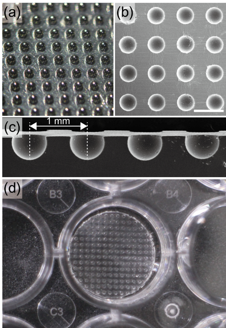
Figure 4: Convex mold and fabricated microwell array. (a) Trapped beads in through-hole array aluminum plate. The trapped beads act as a mold to fabricate the concave microwells. The bead size was 600 \mu\text{m} . The scale bar is 1 mm. (b) and (c) SEM images of fabricated microwells. Each fabricated microwell has a hemispherical shape, 600 \mu\text{m} in diameter. (d) \Phi 14\text{-mm} microwell array in 24-well plate. The array contains over 120 concave microwells. Please click here to view a larger version of this figure.
