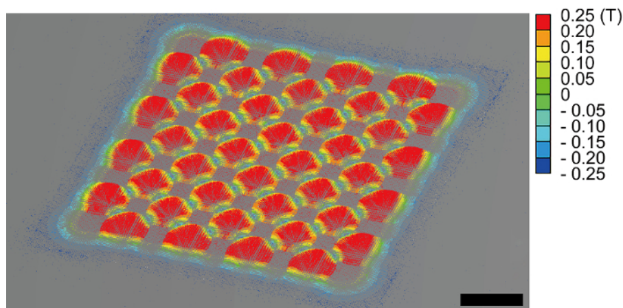
Figure 6: Simulation result for vector of magnetic flux density. The density of the magnetic flux on the magnet array was computed using the magnetostatic module. The simulation result shows that the strongest magnetic flux density is at center of each magnet, causing the beads to be trapped in the center of the through-holes where they became securely fixed. The scale bar is 2 mm. Please click here to view a larger version of this figure.
