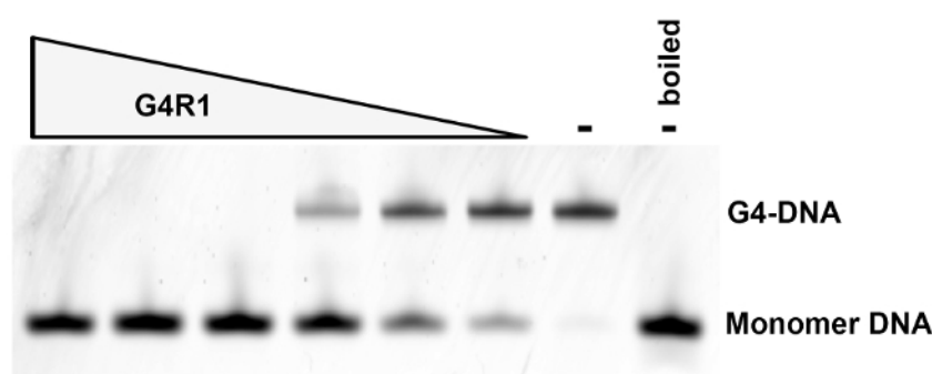
Figure 2: Quality-control G4-DNA Unwinding Assay. Lanes 1 - 6: A constant concentration of TAMRA-labeled tetramolecular G4-DNA was incubated at 37 °C for 30 min in the presence of 4x serial dilutions of purified rG4R1 representing 3.9 \mu L, 0.83 \mu L, 0.2 \mu L, 0.05 \mu L, 0.013 \mu L, and 0.003 \mu L, respectively. Lane 7: tetramolecular G4-DNA in the absence of rG4R1. Lane 8: tetramolecular G4-DNA boiled to reduce the G4 structure into monomers in the absence of rG4R1. Please click here to view a larger version of this figure.
