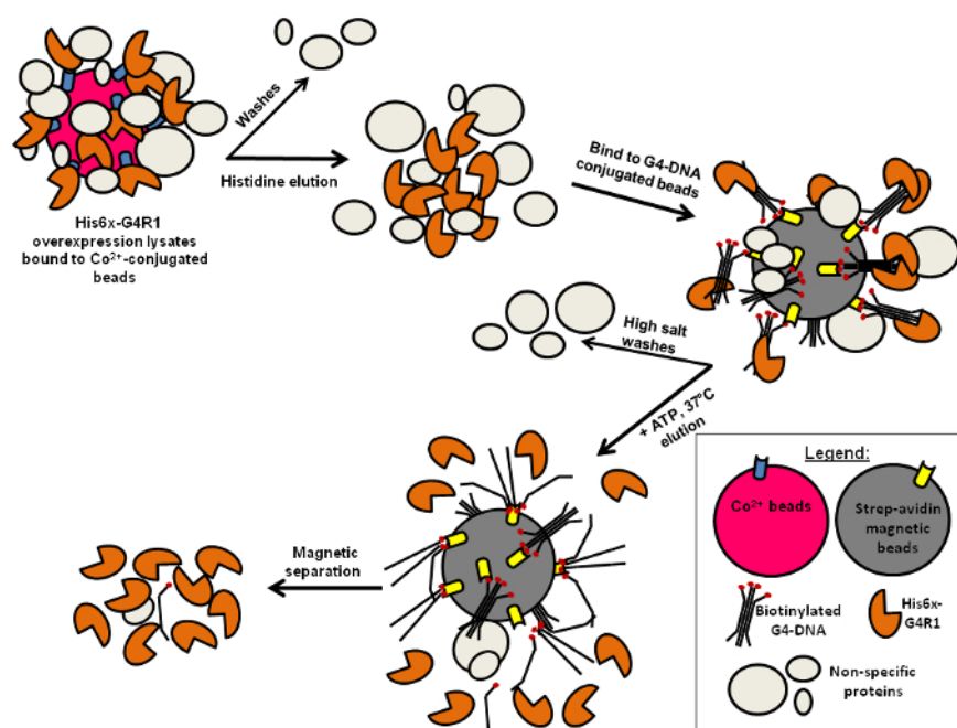
Figure 1: Schematic of a Two-step Purification of G4R1. A 6xHis-tagged rG4R1 is bulk-purified from E. coli lysates by first binding to and eluting from \text{Co}^{2+} -conjugated beads. A binding step to G4-DNA-conjugated magnetic beads follows. Finally, an ATP-dependent elution step is necessary to obtain relatively pure and enzymatically active rG4R1. Please click here to view a larger version of this figure.
