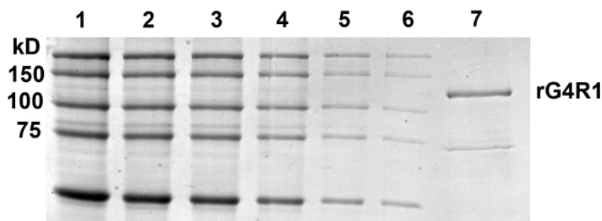
Figure 3: Quantification of Purified rG4R1 Concentration. Broad-range MW protein markers were loaded in the following quantities: 500, 250, 125, 62.5, 31.3, and 15.7 ng in Lanes 1 - 6, respectively, and were used to generate a standard curve of protein concentrations. Lane 7 represents 35 \mu L of rG4R1. This particular gel was quantified, as part of a triplicate set of gels, resulting in an average protein concentration of 62 \pm 22 nM standard deviation (SD; N = 9). Please click here to view a larger version of this figure.
