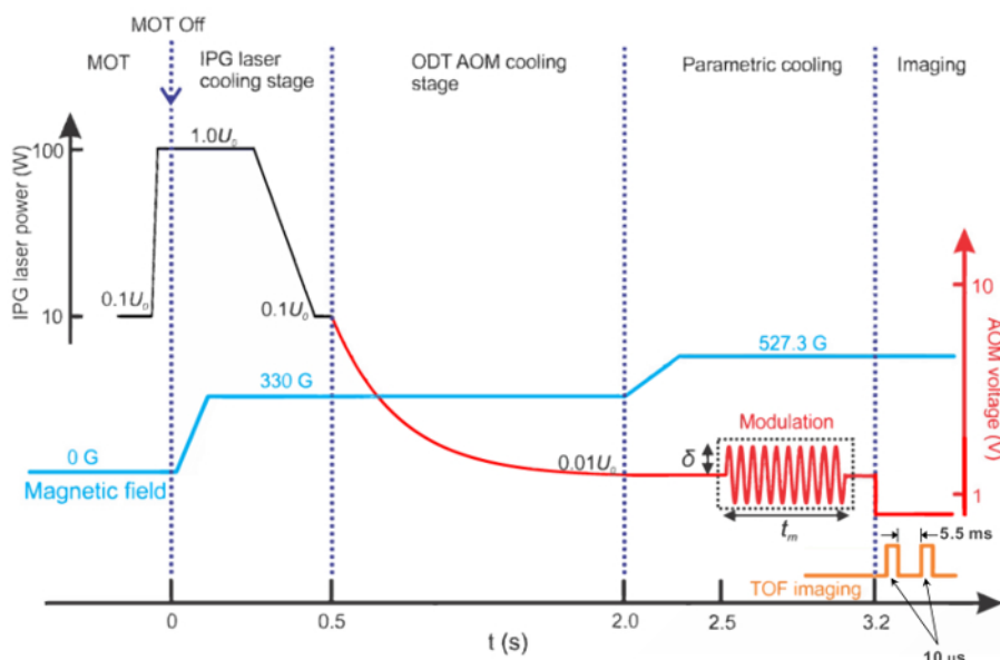
Figure 2: Timing sequence for the parametric cooling. The black curve is the fiber laser power timing. The red curve is one of ODT AOM timing. The cyan curve represents the magnetic field. The orange curve is the TOF imaging pulses. The horizontal axis shows the time scale of each stage. Please click here to view a larger version of this figure.
