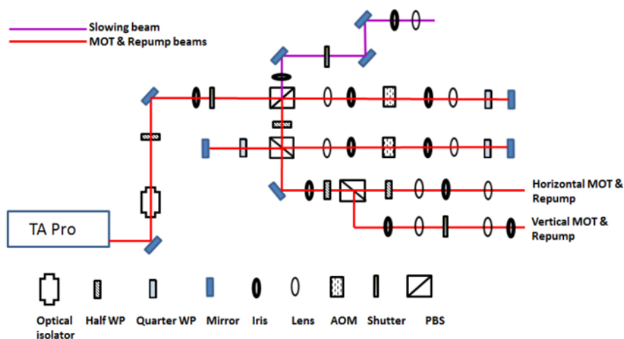
Figure 6: MOT optical layout. The optical setup for generation of the MOT and slowing laser beams. Please click here to view a larger version of this figure.
