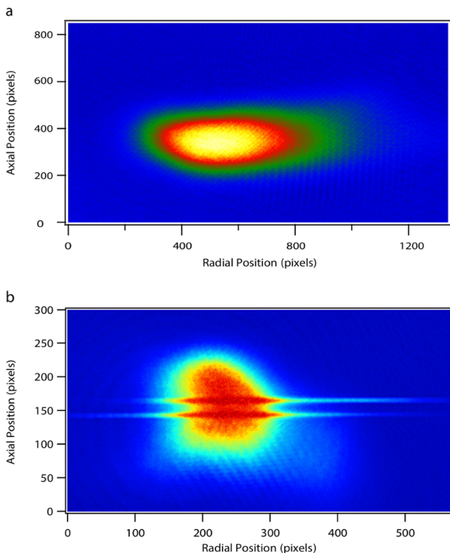
Figure 7: MOT and ODT absorption images. a) MOT image after pumping phase. b) The image of the overlapped MOT and ODT. Please click here to view a larger version of this figure.
