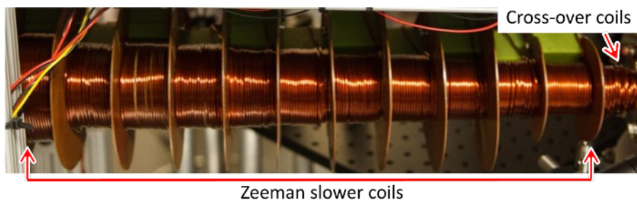
Figure 5: Zeeman slower. The crossover coil is the last section of the Zeeman slower. Please click here to view a larger version of this figure.
