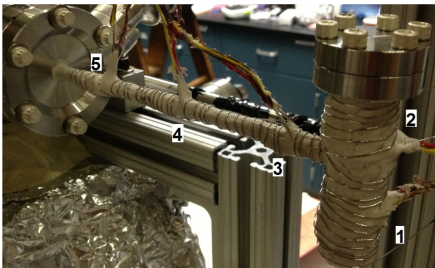
Figure 4: ^6\text{Li} oven. Each labeled section contains a temperature controlled heating coil for the oven to output the required atomic flux. Please click here to view a larger version of this figure.
