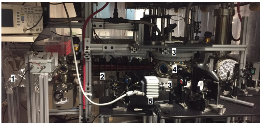
Figure 1: Ultrahigh vacuum system. The vacuum chamber of the ultracold atom apparatus at IUPUI. 1. oven, 2. Zeeman slower, 3. magnet coils, 4. experiment chamber and 5. CCD camera. Please click here to view a larger version of this figure.
