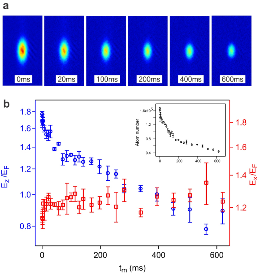
Figure 9: Time dependence measurement of parametric cooling. a) The absorption images of the atomic clouds of various modulation times. b) The dependence of E_{(x,z)}/E_F on modulation time (blue circles are for E_z/E_F and the red squares are for E_x/E_F ). The inset figure is the atom number versus modulation time. Error bars represent one standard deviation. Please click here to view a larger version of this figure.
