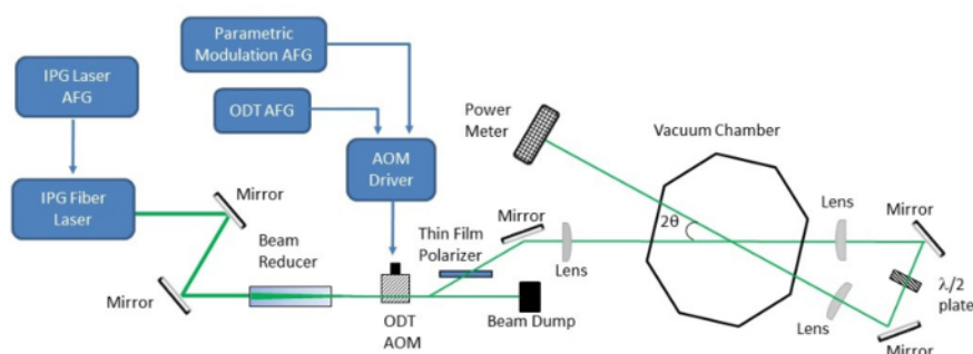
Figure 8: Crossed-Beam ODT optical layout. The crossing angle of the ODT is 2\theta = 12^\circ . The fiber laser AFG controls the pulsing of the laser, the ODT AFG controls the trap lowering curve, and the parametric modulation AFG controls the laser intensity modulation. The beam waist of both beams is about 37 \mu\text{m} . The polarization of the first beam is vertical and the polarization of the second beam is horizontal. Please click here to view a larger version of this figure.
