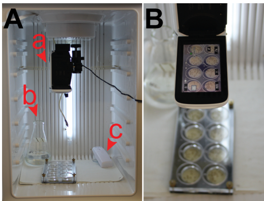
Figure 5: Performing and Recording a 2-D Satiety Assay. (A) A standard consumer camcorder (a) is used to record the assay in an incubator set to the desired temperature. The incubator contains a flask of water (b) and a humidity detector (c) to ensure the appropriate humidity level (>30%). The prepared 2-D satiety assay is filmed under the camcorder (B). Please click here to view a larger version of this figure.
