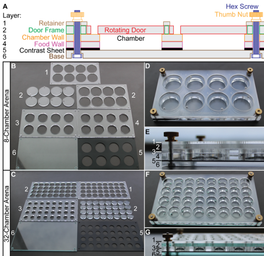
Figure 1. Designing and Assembling Behavioral Arenas. An 8-chamber arena (used for 2-D satiety assays) consists of 6 layers held together by thumb nuts and hex screws ( A ). A 32-chamber arena (used for courtship assays) is manufactured similarly, but without the food wall (layer 4). The arena parts are cut out with a laser cutter and the layers are numbered as ( B ) for 8-chamber and ( C ) for 32-chamber. The assembled 8-chamber arenas are shown in ( D ) (front view) and ( E ) (side view with numbered layers). The assembled 32-chamber arenas assembled in a similar fashion ( F, G ), but Layer 4 (food wall) is omitted ( G ) since no fly food is in the arena for courtship assays. Please click here to view a larger version of this figure.
