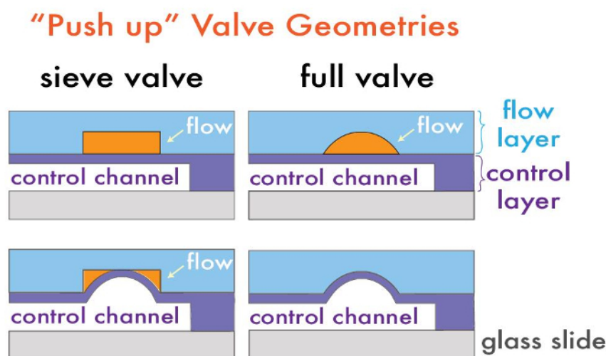
Figure 1: Multilayer Microfluidic Valve Geometries. Typical "push up" device architectures for sieve and fully sealable valves before (top) and after (bottom) pressurization. Please click here to view a larger version of this figure.
