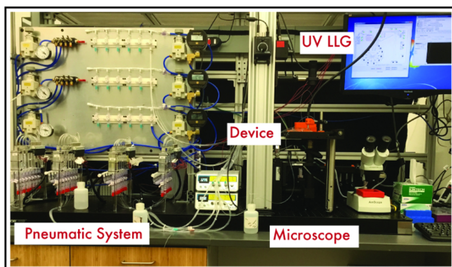
Figure 7: Device operation setup. Image with annotation of all hardware required for device operation. Please click here to view a larger version of this figure.
