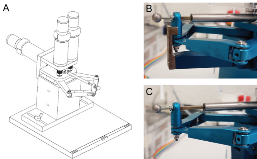
Figure 1: Overview of Robotic Manipulandum and Handle Positioning. (A) Technical drawing showing the robotic manipulandum and marks for alignment with the training cage. (B) Handle held in constant reference position at the start of a training session. (C) Handle in free starting position at the start of a pulling trial. Please click here to view a larger version of this figure.
