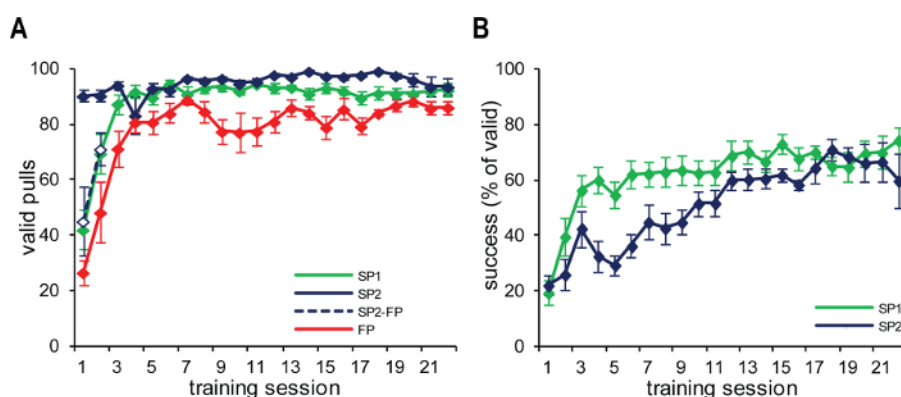
Figure 2: Typical Learning Curves of a Reach-and-pull Task. (A) Valid pulling attempts in a free pull task (FP, N = 6), straight pull task without introductory FP-sessions (SP1, N = 12) and a straight pull task (SP2, N = 7) with introductory FP-sessions (SP2-FP). Values are mean \pm S.E.M. (B) Successful pulling attempts as percentage of valid attempts in the straight pulling task with (SP2) and without (SP1) introductory FP-sessions. Values are mean \pm S.E.M. Please click here to view a larger version of this figure.
