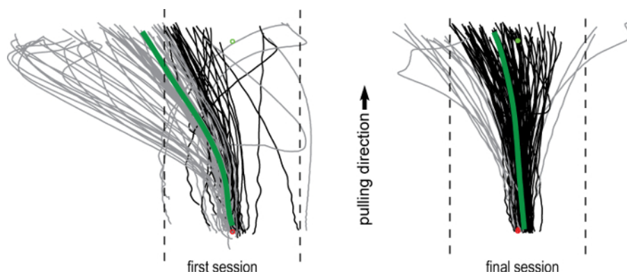
Figure 3: Pulling Trajectories become Progressively Straighter and Less Variable Throughout Training of the SP2 Task. Successful (black), failed (grey) and average (green) trajectories are shown for the first and final straight pull training session for a representative animal. Dotted lines show the 4 mm wide zone within which a successful trial is executed. The red dot denotes the starting position of the handle. The green dot shows the theoretical endpoint of a perfectly straight 10 mm pulling attempt. Please click here to view a larger version of this figure.
