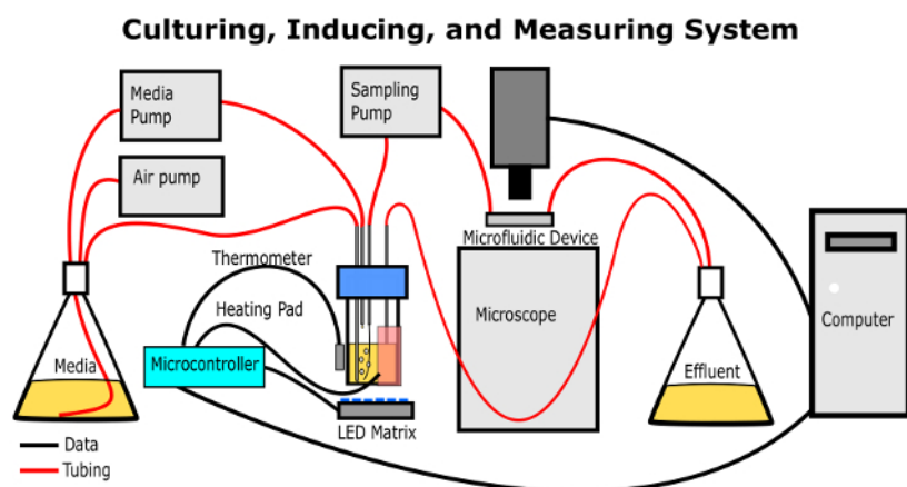
Figure 1: The continuous culturing apparatus. This simplified diagram shows how the apparatus should be assembled when it is used to culture, illuminate, and measure optical properties of the microbes. Please click here to view a larger version of this figure.
