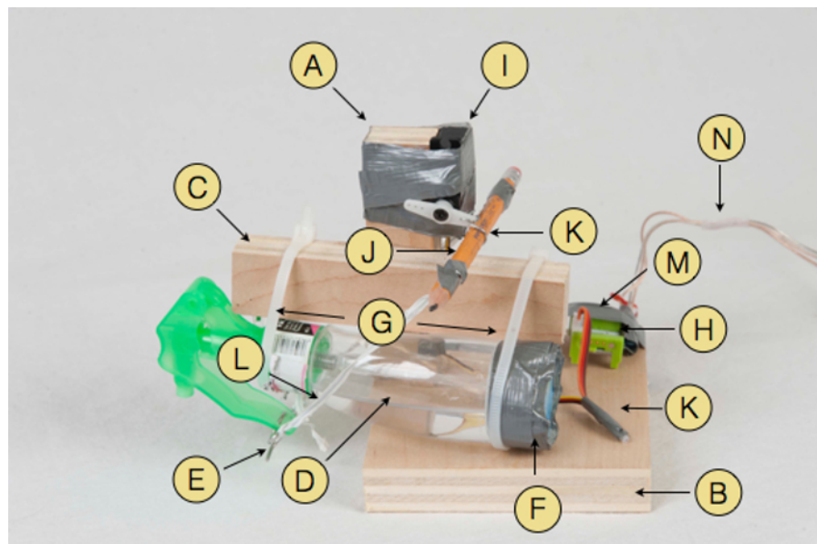
Figure 1: Photograph of the Nebulizer. Parts used: Wooden structure parts (A, B, C), spray bottle (D), bent steel rod (E), duct tape (F), plastic cable ties (G), 011 servo connector part (H), servo motor (I), pencil (J) held by bent paper clip (K), plastic covered wire twist ties (L) w/ wire connector (M) and speaker cable (N) leading to the battery. This figure is based on research originally published in reference 19 . Please click here to view a larger version of this figure.
