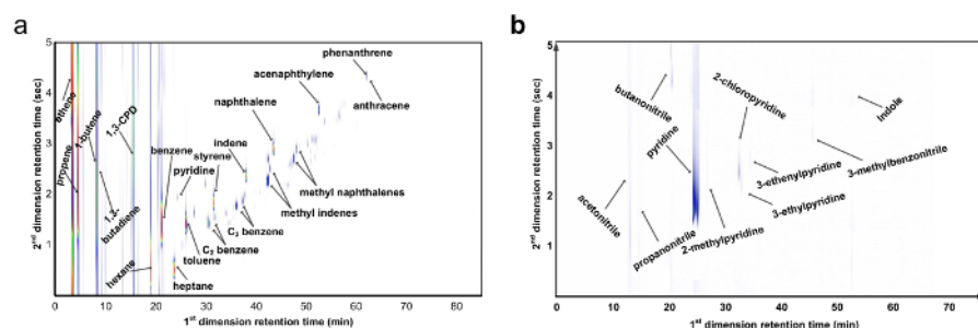
Figure 6. Product analysis during steam cracking of heptane with traces of pyridine. (a) GC x GC-FID chromatogram (b) GC x GC-NCD chromatogram. Detection of major steam cracking products with FID and minor nitrogen containing steam cracking products with NCD. The experiment is performed with steam dilution of 0.5 kg/kg, a COT of 1,123 K, and a COP of 170 kPa. Please click here to view a larger version of this figure.
