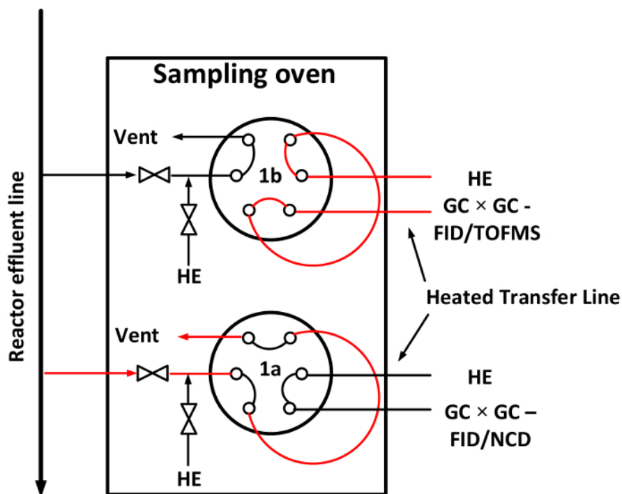
Figure 1. Detailed schematic representation of the GC \times GC sampling oven and valves. Valve 1a is shown in the purging position, flushing the sample loop with effluent. Valve 1b is shown in injection position; carrier gas (helium) is rerouted to the sampling oven, where it is used to transport the effluent sample to the respective GC via a transfer line 18 . Please click here to view a larger version of this figure.
