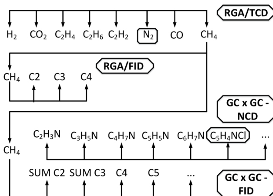
Figure 2. Schematic representation of the quantitative on-line effluent analysis method using a reference compound. The known amount of nitrogen added to the effluent stream is detected on the RGA/TCD and used to determine the concentration of methane which is a reference compound for reactor effluent analysis. Similarly a known amount of 2-chloropyridine is added to the effluent stream and used as internal standard for GC \times GC–NCD analysis. Please click here to view a larger version of this figure.
