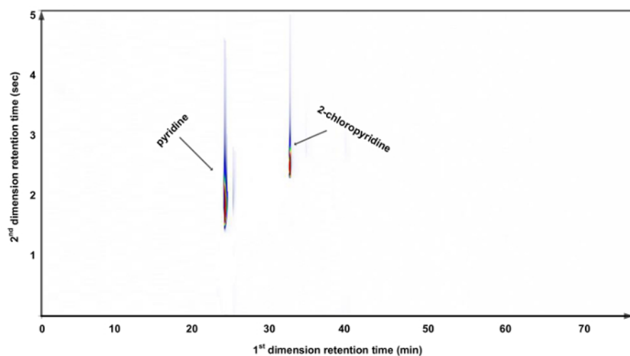
Figure 5. GC x GC-NCD on-line detection of pyridine in the reactor effluent stream under non-reactive conditions. The experiment is performed isothermally at 773 K and a COP of 170 kPa and used for the evaluation of the internal standard quantification method. Please click here to view a larger version of this figure.
