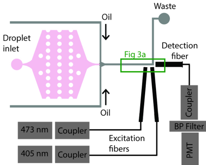
Figure 2. Device design and optical layout. The fluidic portions of the device are comprised of a droplet reinjector and an oil spacer, coupled to an L-shaped channel. Fibers coupled to individual lasers are inserted normal to the direction of flow. A detection fiber is inserted perpendicular to the laser fibers in order to collect fluorescent light. This light is filtered through a bandpass filter, before being detected by a single PMT. Please click here to view a larger version of this figure.
