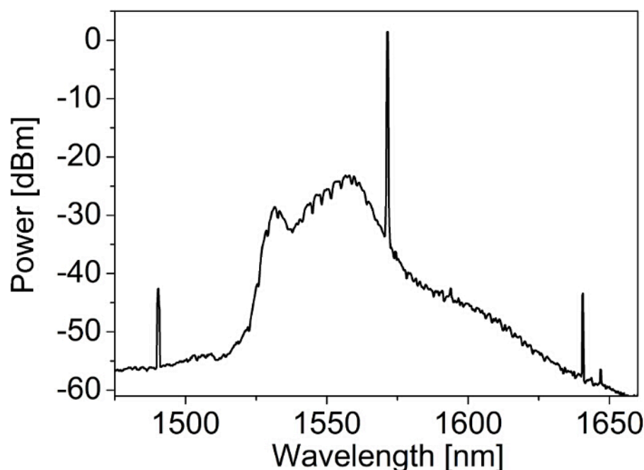
Figure 9. Perfect Phase Matched SRS-SARS. Experimental spectrum of SRS and SRS perfectly phase matched with a SARS-SRS intensity ratio close to 1. The microsphere diameter is 65 \mu\text{m} . Please click here to view a larger version of this figure.
