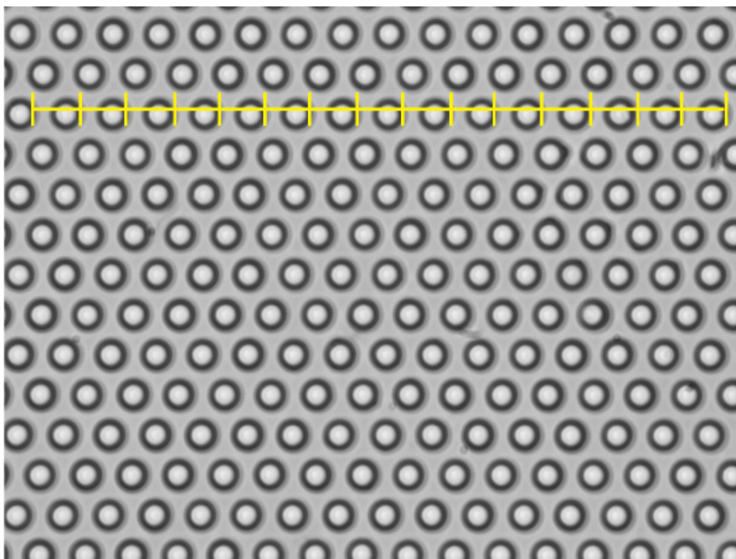
Supplementary Figure 9. The pixel size for a microscope setup is typically determined using a special microscope slide with a scale bar on it; alternatively the micropost array layout, given by the manufacturer can be used. For example, 15 units with 13 microns (195 \mu\text{m} total length) divided by 2,375 pixels (established with an image processing tool) leads to 0.082 \mu\text{m}/\text{pxl} . Please click here to view a larger version of this figure.
