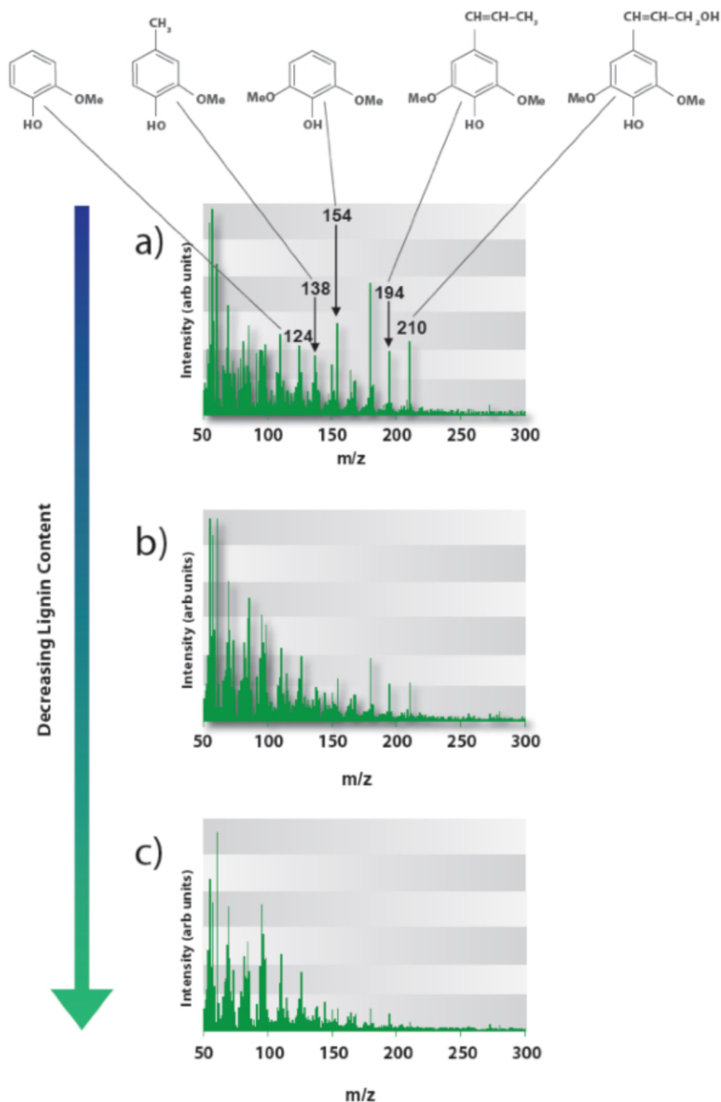
Figure 5: Application of pyMBMS for the analysis of chemical changes in plant cell walls 28 . The peaks denoted with arrows are lignin fragments, and were used to evaluate (a) high lignin (b) medium lignin or (c) low lignin content.
