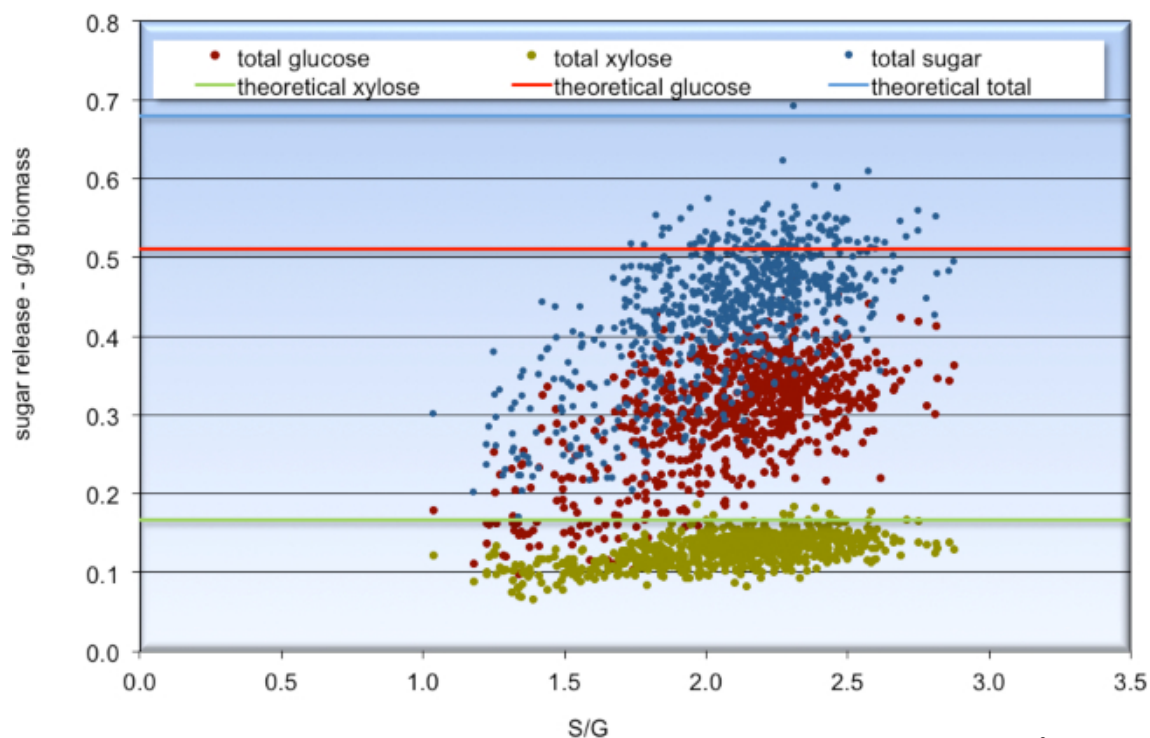
Figure 2: Recalcitrance of poplar cell walls as a function of syringyl to guaiacyl (S/G) content in lignin 9 . Increasing the recalcitrance of poplar cell walls as a function of syringyl to guaiacyl (S/G) content in the lignin fraction has been observed and reported. 755 poplar core samples of the same poplar cultivar were taken over several hundred miles of forest in the North American Pacific Northwest and screened for glucose and xylose release after thermochemical pretreatment and enzyme saccharification. Results were plotted against the S/G ratio in the cell wall lignin as determined by pyMBMS. Recalcitrance decreases with increasing S/G until about 2, where it remains constant at higher S/G. Theoretical yield values are based on the BESC “standard” poplar and are provided as a reference for comparison.
