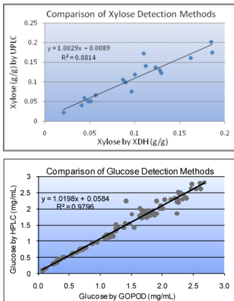
Figure 1: Comparison of glucose and xylose quantitation using high-throughput colorimetric assays vs. HPLC 9 . Comparison of glucose and xylose detection was carried out using Xylose DeHydrogenase (XDH, top panel) and Glucose Oxidase/Peroxidase (GOPOD, lower panel) high-throughput colorimetric enzyme-linked assays and high-performance liquid chromatography.
