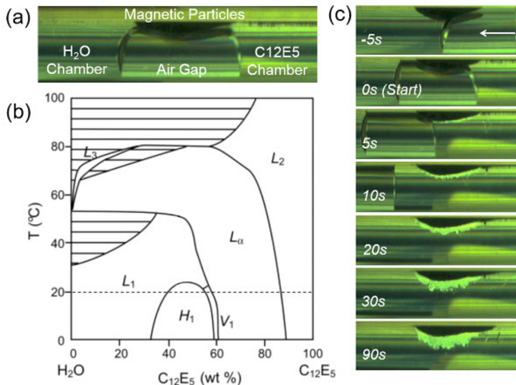
Figure 3. (A) Lab-in-tube experimental setup. (B) Phase change plot of the H 2 O/C12E5 binary system. (C) Observed phase change of H 2 O/C12E5 from 0 to 90 sec. Reprinted (adapted) with permission from Blumenschein, N., Han, D., Caggioni, M., Steckl, A. Magnetic Particles as Liquid Carriers in the Microfluidic Lab-in-Tube Approach To Detect Phase Change. ACS Applied Materials & Interfaces. 6 (11), 8066-8072, doi: 10.1021/am502845p (2014). Copyright 2014 American Chemical Society. Please click here to view a larger version of this figure.
