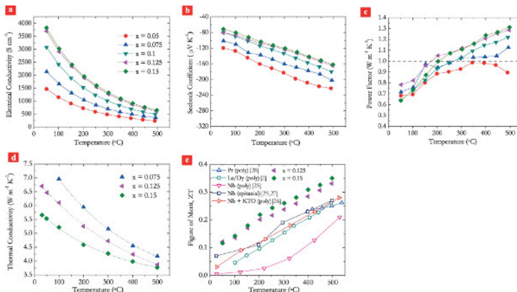
Figure 3. Thermoelectric transport properties. Temperature dependence of (A) electrical conductivity ( \sigma ), (B) Seebeck coefficient ( \alpha ), (C) power factor (defined as PF = \alpha^2 \sigma T ), (D) total thermal conductivity and (E) figure-of-merit, ZT for Sr_{1-x}Pr_xTiO_{3-\delta} ceramics as a function of Pr content. Temperature dependence of reported maximum ZT values in the literature is shown for comparison. 2,25-28 Reproduced with permission. 12,13 Please click here to view a larger version of this figure.
