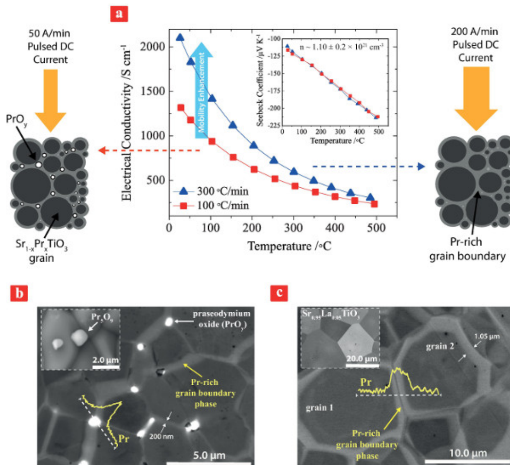
Figure 2. Effect of SPS heating rate. (A) Temperature dependence of electrical conductivity and Seebeck coefficient (inset) for \text{Sr}_{1-x}\text{Pr}_x\text{TiO}_{3-\delta} ceramics with x = 0.075 processed using two different SPS heating rates of 100 ^{\circ}\text{C min}^{-1} and 300 ^{\circ}\text{C min}^{-1} , respectively. (B) Backscattered electron (BSE) micrograph of the ceramic made under 100 ^{\circ}\text{C min}^{-1} SPS. A typical Pr spectrum of the EDS line scan across a \text{PrO}_y particle is shown. (C) Backscattered electron micrograph of the ceramic made under a 300 ^{\circ}\text{C min}^{-1} SPS heating rate. A typical Pr spectrum of EDS line scan across two grains, grain 1 and grain 2, is shown. The inset depicts the BSE micrograph of the \text{Sr}_{0.95}\text{La}_{0.05}\text{TiO}_3 ceramic prepared following the same recipe. Reprinted with permission. 12 Please click here to view a larger version of this figure.
