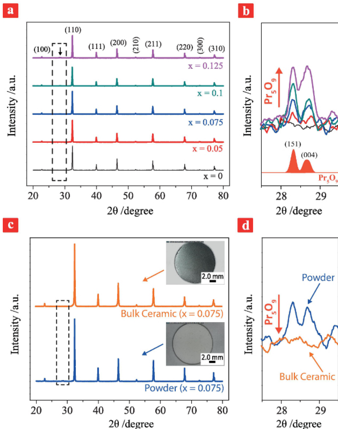
Figure 1. X-ray diffraction profiles. (A) X-ray diffraction (XRD) profiles of \text{Sr}_{1-x}\text{Pr}_x\text{TiO}_{3-\delta} powders before SPS as a function of nominal Pr content. (B) Magnified view of the dashed rectangle in (a), (C) XRD profiles of \text{Sr}_{1-x}\text{Pr}_x\text{TiO}_{3-\delta} with x = 0.075 before SPS (Powder) and after high-heating-rate SPS (Bulk Ceramic). Photographs of cold-pressed powder after solid-state reaction and the corresponding SPSed ceramic are shown. (D) Magnified view of the dashed rectangle in (C). Reprinted with permission. 12 Please click here to view a larger version of this figure.
