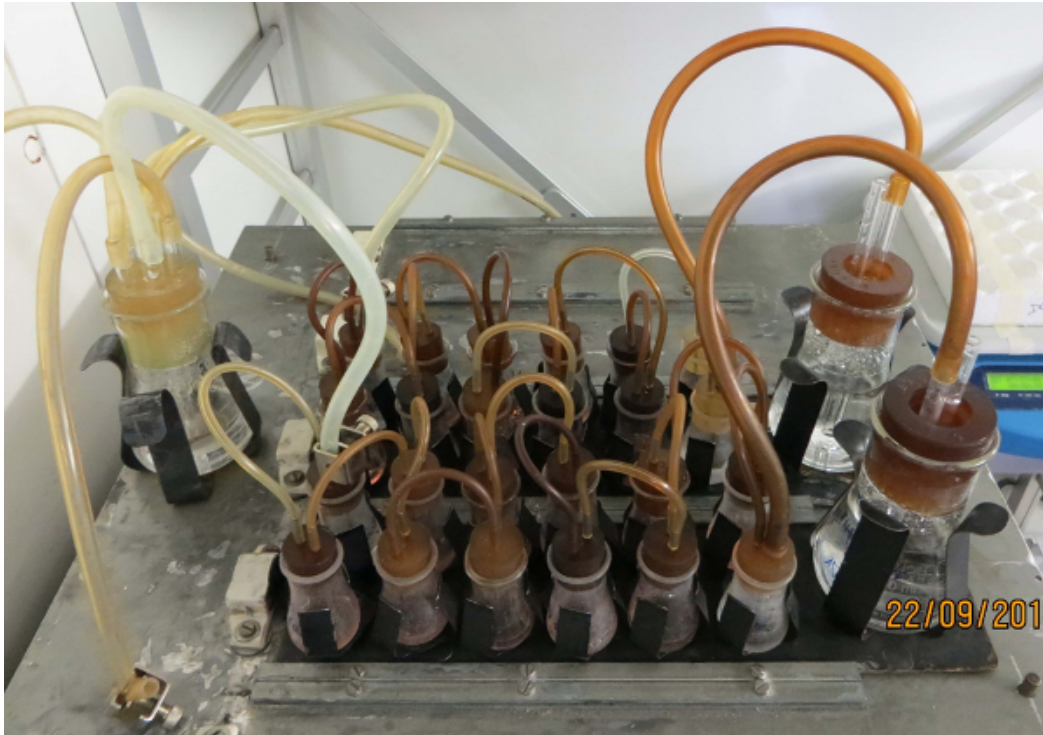
Figure 4. Small Erlenmeyer flasks on top of a gyrotory shaker. The flasks with 1.5 ml of culture medium are sealed with silicone stoppers equipped with a gas in - and outlet needle, and moved at 120 rpm at 37 °C. The gas is led by an inlet tubing (1) to the larger Erlenmeyer flask (2) filled with sterile Ringer's salt solution, and further distributed (3 and 4) to smaller flasks containing culture medium with individual confronting pairs (5 and 6). Finally, spent gas is collected in a larger flask with a sterile water trap (7), from where it can escape into the air (8). The figure shows two sets of culture batteries on top of a home-made platform plate. Please click here to view a larger version of this figure.
