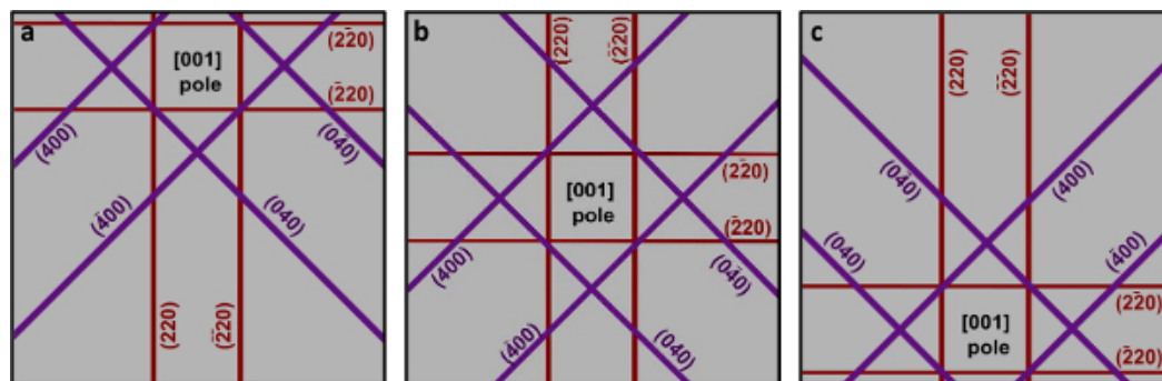
Figure 3. Tilt of Electron Channeling Pattern (ECP). Depiction of the effect of out-of-plane sample tilt ( i.e. , about the in-plane [110]) on the appearance of the GaP/Si ECP. Tilts of (A) -4^\circ , (B) 0^\circ , and (C) 4^\circ are shown. Please click here to view a larger version of this figure.
