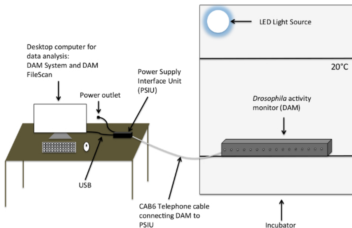
Figure 5. Diagram illustrating the Drosophila Activity Monitor set-up and its connectivity to the PSU interface unit and a desktop computer. The inside of the incubator is depicted, but during recording the incubator is to be shut.
