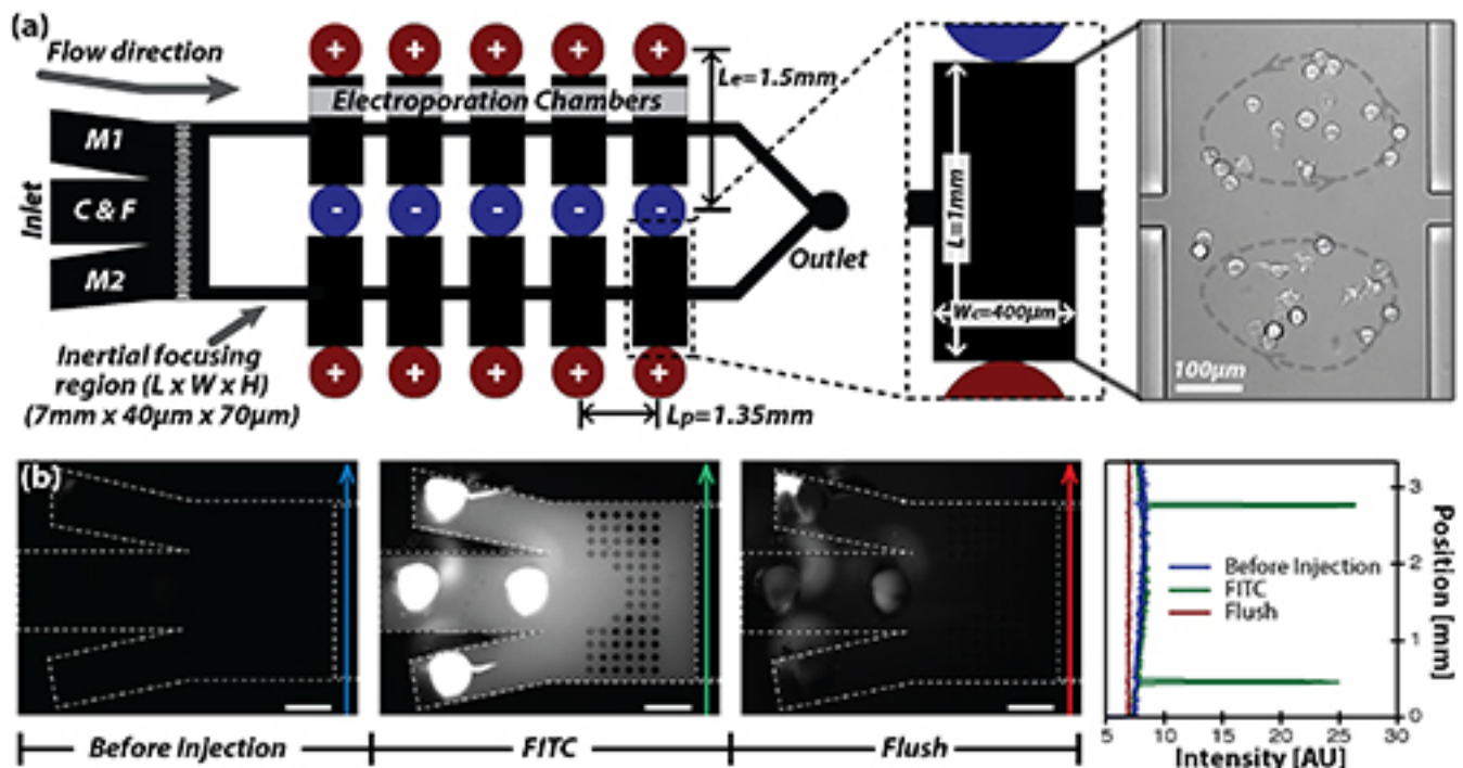
Figure 1. (A) A schematic of the microfluidic electroporation system, consisting of inlets for cells (denoted as C), molecules (denoted as M1 and M2) and a flush solution (denoted as F), two straight channels where inertial focusing occurs, 10 electroporation chambers with electrodes and an outlet. (B) Solution exchange demonstration at the inlet using a 1 \mu M FITC solution and a flush solution (DPBS) indicates that the active solution can be uniformly injected to all arrays of chambers downstream. Image contrast is enhanced by adjusting look-up table (LUT). Scale bars are 250 \mu m. Please click here to view a larger version of this figure.
