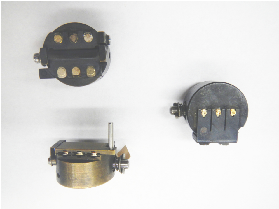
Figure 4. Two types of specimen mounts for freeze-fracture/etch procedures. (Left) A double replica specimen holder booklet is used for conventional freeze-fracture procedures performed without etching. The specimen is sandwiched between two gold specimen stubs and positioned in the brass booklet. The specimen is fractured by opening the booklet under vacuum in the specimen chamber (See freeze-fracture_movie1.mov). (Right) A mount used primarily for freeze-etching. The specimen is positioned on the gold stubs and locked into the brass holder. The specimen is fractured by gentle shaving with a razor blade fixed in the microtome arm. This configuration is preferred for etching procedures (See freeze-etch_movie2.mov).
