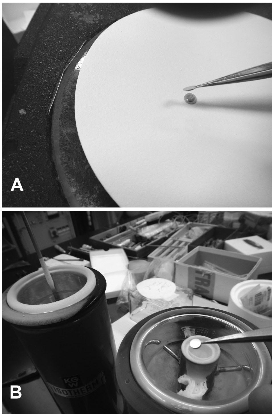
Figure 5. Preparation of a freeze-fracture specimen mount. The specimen is sandwiched between two gold mounts (A) and frozen in a well containing liquid nitrogen cooled propane (foreground) with subsequent transfer to a holding Dewar containing liquid nitrogen (background) (B).
