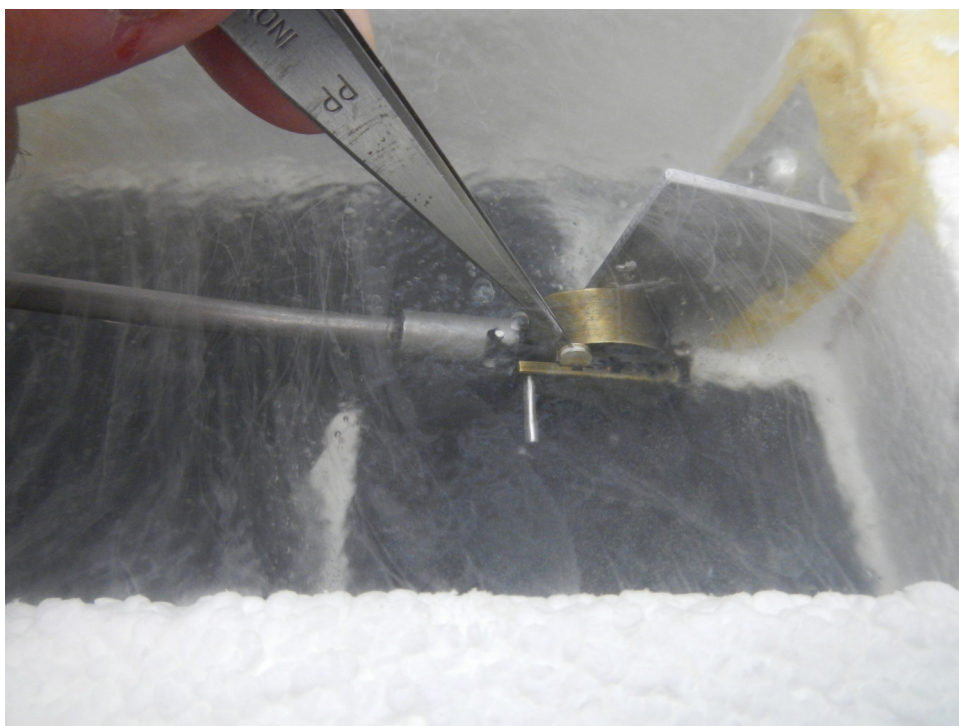
Figure 6. Demonstration of positioning of a frozen freeze-fracture specimen into the double replica specimen holder booklet in preparation for introduction to the specimen chamber of the freeze-fracture/etch plant.
