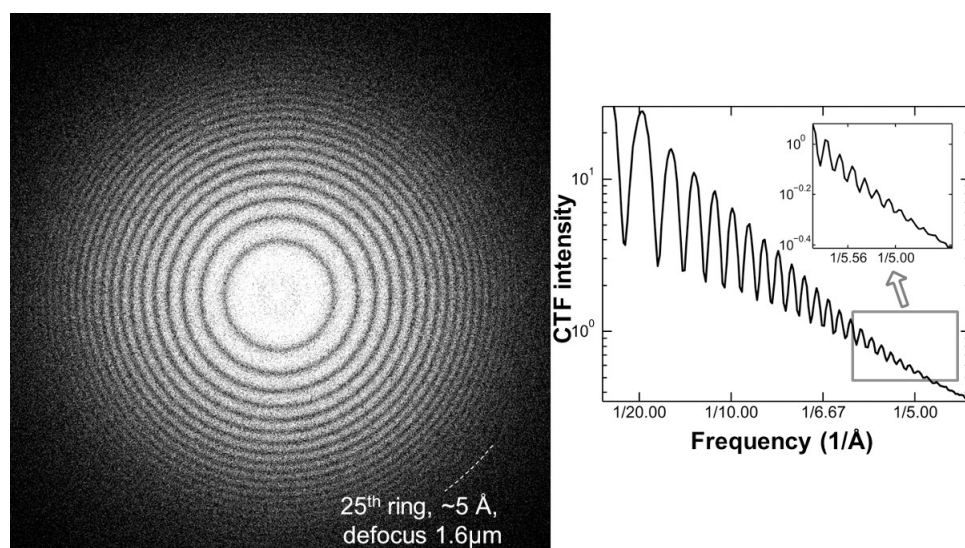
Figure 5. Power spectrum of amorphous carbon film imaged under 1.6 \mu\text{m} defocus by a Zeiss Libra 120 LaB6 TEM. High-resolution imaging requires sufficient evidence to show that EM has the proper alignment and high-resolution capability. The analysis of the power spectrum of nearby carbon area on the grid is an efficient method to check the beam coherence condition prior to data acquisition. Fourier transfer of the image of an amorphous carbon area show the instrument related contrast transfer function (CTF), so called Thon-rings. A proper alignment and coherence can be reflected by the number of visible Thon-rings and the highest resolution of visible Thon rings under a relatively high defocus condition. As an example of a near proper alignment condition of a LaB 6 filament equipped TEM, more than ~20 Thon rings (~5 Å) can be generated from a carbon film are imaged at 1.6 \mu\text{m} defocus using dose 20.4 \text{e}^-/\text{Å}^2 . The Thon rings achieved from a low-end TEM have a similar to that from high-end TEM, such as a field-emission gun (FEG) enhanced TEM operated under a proper alignment condition. This work initially published in Scientific Reports 5 . Please click here to view a larger version of this figure.
