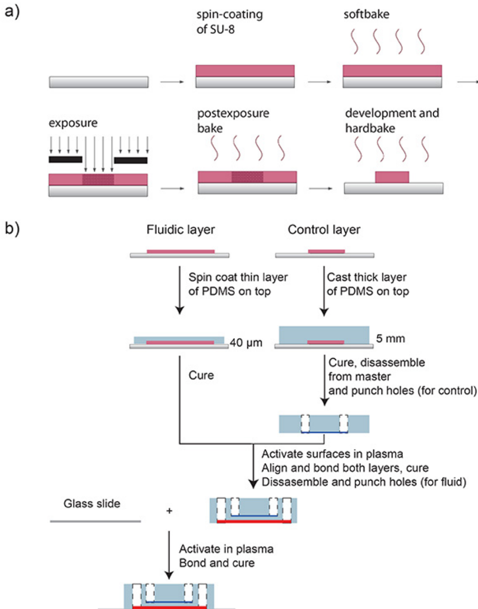
Figure 3. Schematic of of SU-8 processing and PDMS production. a) Schematic of the SU-8 processing protocol. A silicon wafer is spin-coated with SU-8 and soft-baked at 95 °C for 4 min. The desired microfluidic channel design is transferred onto the SU-8 using a photomask and UV-light exposure. After a post-exposure bake (95 °C, 5 min), SU-8 is developed and hard-baked at 180 °C for 2 hr. b) Schematic of the microfluidic chip fabrication. A mixture of PDMS oligomer and curing agent is spin-coated onto the master form for the fluidic channels, and poured onto the master form for the control layer. The channel negatives are depicted in pink. Both layers are cured in an oven. The control layer chip part is disassembled from the wafer (control channel in blue) and holes for the pressure connections are punched (white). Both parts – control and fluid layer- are placed in oxygen plasma, and afterwards, they are aligned and bonded. The whole chip is then disassembled from the fluidic master form (fluid channel in red) and fluidic access holes are punched (white). Finally, the chip and a glass slide are bonded after surface activation in oxygen plasma. Click here to view larger image.
