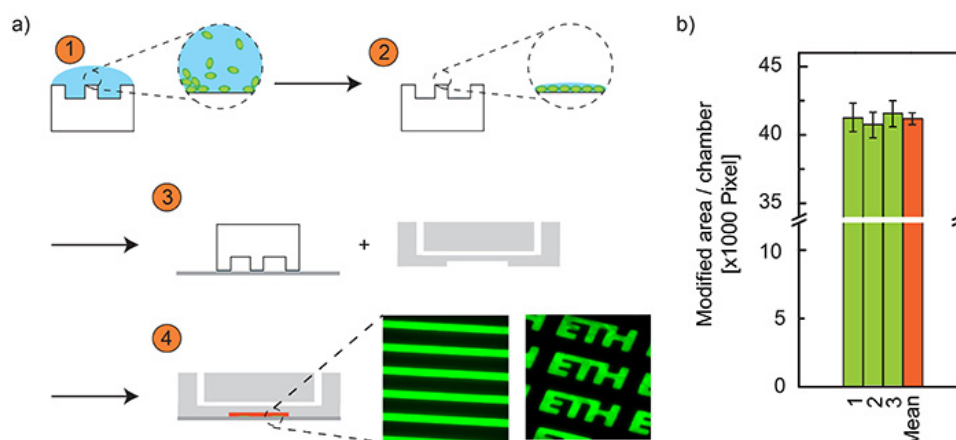
Figure 4. Schematic of the microcontact printing. a) Master fabrication for soft lithography. (1) A PDMS stamp is incubated with protein (bBSA) solution. (2) The solution is removed, the stamp is washed and a monolayer of protein remains on the stamp. (3) The stamp is placed on a glass slide, thereby the proteins are transferred to the glass surface. During this time, the microchip together with the stamp on the glass are exposed to an oxygen plasma. (4) The stamp is removed and the microchip is bonded to the glass slide. For visualization, two example structures are shown, printed with fluorescent BSA-fluorescein conjugate. b) Microcontact printed area per chamber. Since printing and chambers are not aligned, we evaluated the variations on binding spots (printed area) on three different chips (numbers 1-3) and all 60 microchambers. As a result, chamber-to-chamber variability is relatively small (<2.5%) and chip-to-chip variability was negligible (<1%), demonstrating that there is indeed no need to align the printed structures to the chambers. Click here to view larger image.
