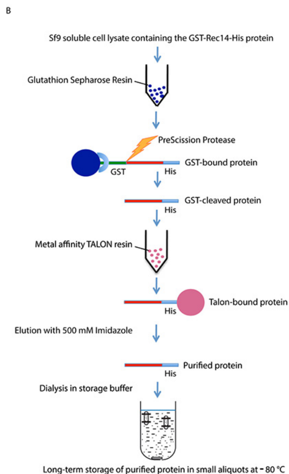
Figure 1. Schematic outline of the GST-His two-step affinity purification method. A. GST-Rec14-His construct cloned into pFastBac (Baculovirus expression vector). B. Two-step affinity purification of GST-Rec14-His from Sf9 soluble cell lysate: GST-binding, followed by PreScission cleavage of the GST, TALON-binding and elution with imidazole. Click here to view larger figure.
