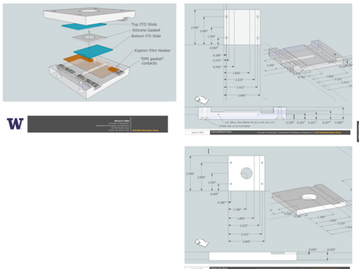
Figure 5. Plans for electroformation chamber. Included is an overview, showing the complete assembly, and dimensioned schematics for the top and bottom plastic pieces. Use acrylic or another easily machined clear plastic. The thin Kapton film heater should be connected to the temperature controller (see Table of specific reagents and equipment), and the EMI gasket foam should be connected to the function generator, so that the sine wave signal is applied across the two ITO coated slides. A hole is provided for a temperature probe. Flathead 10-32 screws are placed in the countersunk holes in the bottom piece, and pass through the upper piece. 10-32 nuts are used to secure the assembly. When fully assembled, the top and bottom plastic pieces should be flush with each other on two sides (the sides parallel to the EMI gasket.) Click here to view larger figure.
