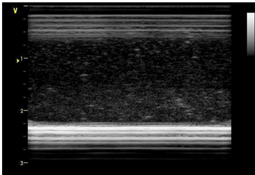
Figure 2. Raw ultrasound B-mode image of pipe flow. The high intensity band of lines at the top and bottom of the image correspond to the pipe wall and the ellipsoids interior to the wall correspond to the 10 \mu m hollow glass microspheres.
