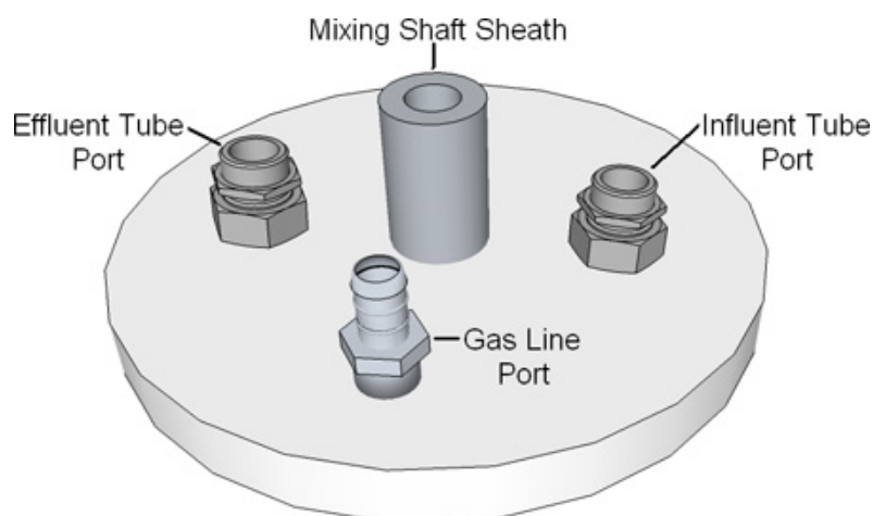
Figure 2. Basic example of reactor lid design: Lid material- PVC/Plexiglas; Fittings material- Stainless Steel/Plastic; Tubing material- Stainless Steel/Aluminum.
