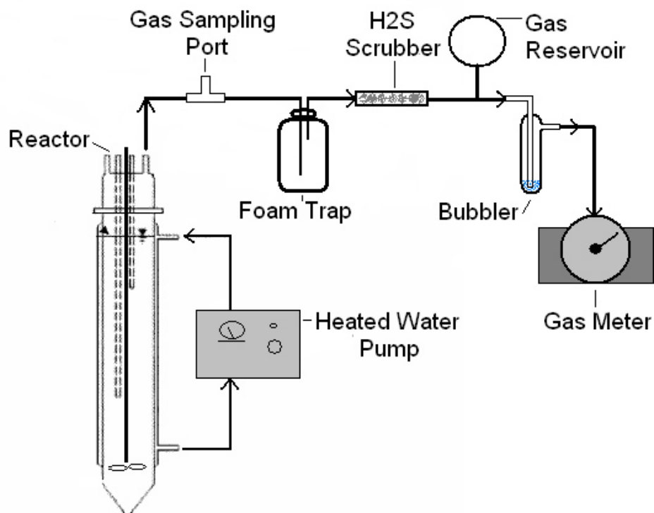
Figure 3. System diagram showing component arrangement.
