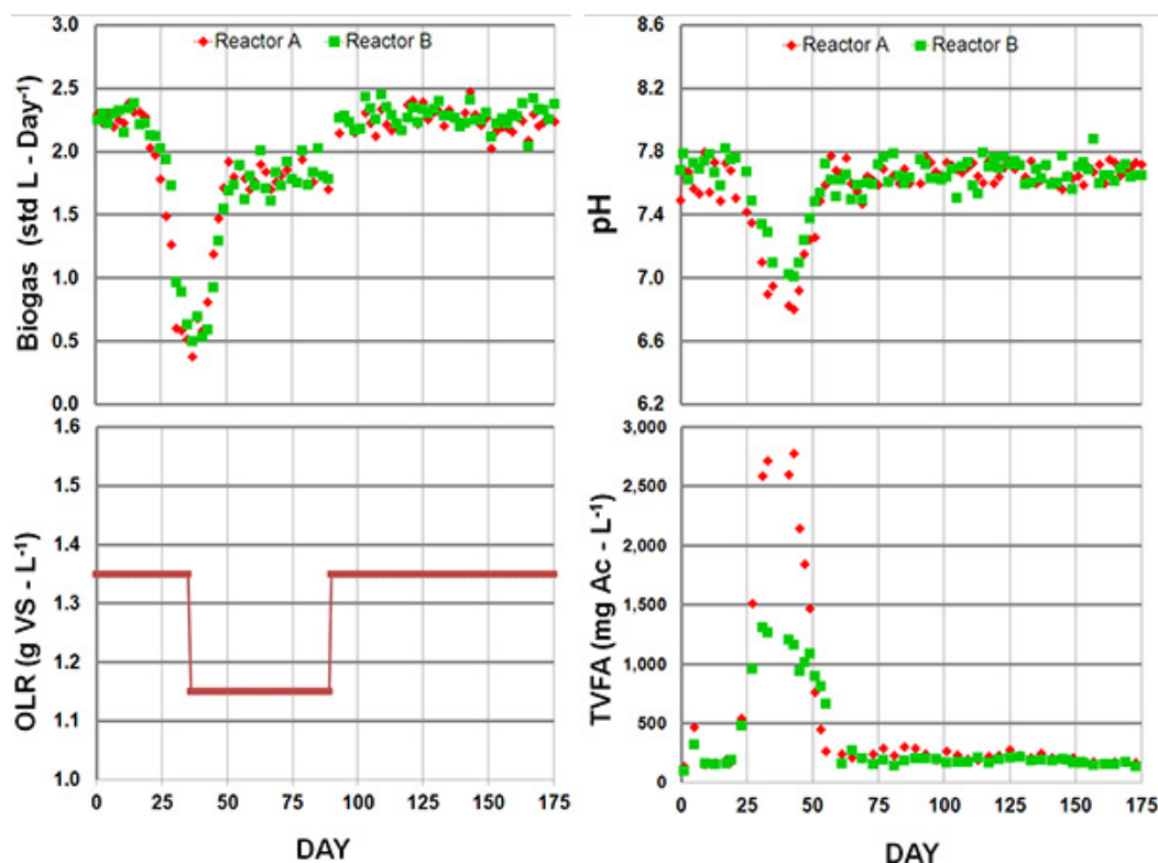
Figure 5. Typical system response to a high organic loading rate (OLR) during reactor start-up. Beginning with an OLR of 1.35 gVS-L -1 caused the accumulation of total volatile fatty acids (TVFA). The acid accumulation caused a decrease in pH followed by a reduction in biogas yield. By lowering the OLR to 1.15 g VS-day -1 , both systems were able to recover and establish a sufficient methanogenic biomass concentration to tolerate a 1.35 gVS-L -1 OLR. The difference in pH and TVFA accumulation between reactors exhibits the unique dynamics of mixed communities.
