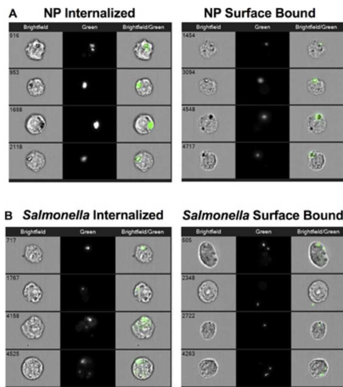
Figure 2. Cell images of internalized and surface bound nanoparticles (NP) or Salmonella . (A) Representative images of RAW 264.7 cells that internalized NP (left panel) and cells to which NP were bound to their surface but not internalized (right panel). (B) Representative images of RAW 264.7 cells that internalized Salmonella (left panel) and cells to which Salmonella were bound to their surface but not internalized (right panel).
