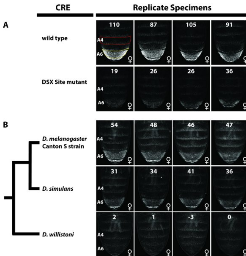
Figure 3. Quantitative comparison of cis -regulatory element activities. For all samples EGFP-reporter gene expression mediated by a particular Dimorphic Element was assessed in females at 80 hours after puparium formation. The number at the top of each image is the EGFP-expression level for the specimen that is calculated as the mean pixel value for the A6 abdominal segment (indicated for the upper left most image as the region within the dashed yellow border) minus the mean pixel value for the A4 segment (background correction; indicated for the upper left most image as the region within the dashed red border). For each reporter transgene four replicates were assessed to calculate a mean segment A6 pixel value. Regulatory activity is reported as the % of the (A) wild type or (B) Canton S strain female mean pixel value \pm SEM. (A) GFP expression for females possessing a wild type allele of the Dimorphic Element and a mutant version where a single binding site for the DSX transcription factor was ablated. This mutant binding site reduced Dimorphic Element activity to 28 \pm 3\% of the wild type sequence. (B) Comparison of the regulatory activities for sequences orthologous to the D. melanogaster (Canton S strain) Dimorphic Element. Considering the GFP expression mediated by a D. melanogaster Dimorphic Element allele as 100%, the orthologous sequences from the related species D. simulans and D. willistoni respectively possess activities of 75 \pm 4\% and 0 \pm 0\% .
