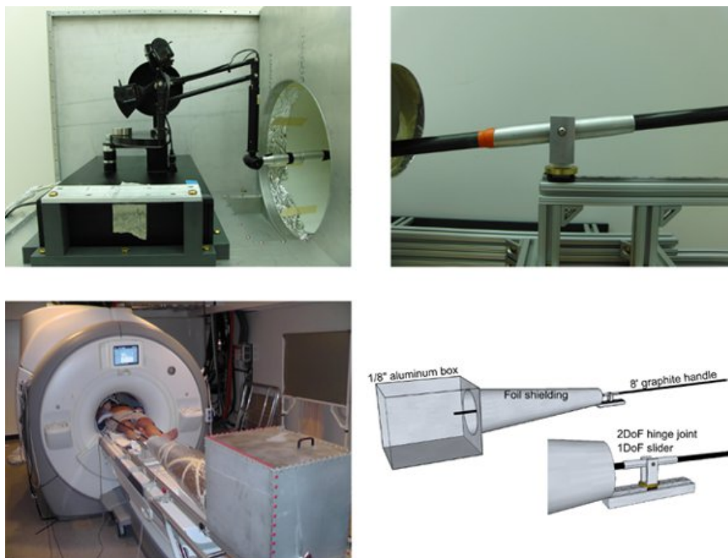
Figure 1 The apparatus used to mount the haptic robot for use in the fMRI environment. Top shows the haptic robot mounted in the case prior to enclosure (top, left) and the gimbal/slider joint at the midpoint of the handle (top, right). Bottom, left shows a subject in the scanner manipulating the handle. Bottom, right is a cartoon of the shielding and end effector.
