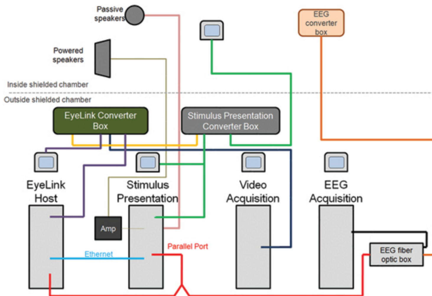
Figure 5: Cabling diagram of the laboratory setup.
