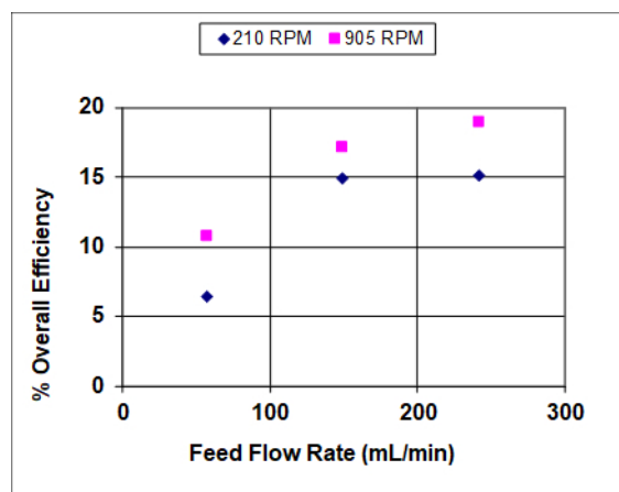
Figure 4: Percent overall stage efficiency for IPA extraction using a York-Scheibel column, 11 stages, 16 - 18 mol% IPA in hydrocarbon mixture (feed), S/F (molar) = 1.5.
