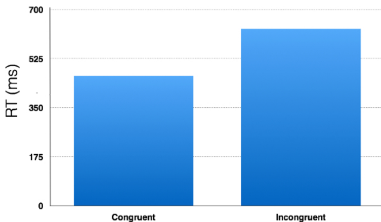
Figure 4. Reaction time results of a spatial cueing experiment. Participants generally responded more quickly in congruent compared to incongruent trials. In congruent trials, the cue arrow pointed to the place where a letter eventually appeared. But in incongruent trials, it pointed opposite. The difference in reaction times suggests that the arrow led participants to attend to the box pointed to by the arrow, allowing them to more quickly process and identify the letter when it appeared there.
