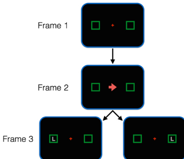
Figure 1. Sequence of events in the spatial cueing paradigm used to measure the consequences of visual attention. Each trial begins the same way, as shown in frame one, with a central fixation cross and two green boxes on either side. In frame two, the fixation cross is replaced by an arrow, pointing to one of the two boxes (50% of the time each). Finally, in frame three a letter is shown—either an L or a T—in one of the two boxes. In the example shown, the letter is an L. In the right panel example, the letter appears in the box that the arrow points to, producing a congruent trial. In the panel on the left, the letter appears opposite the arrow, producing an incongruent trial. The measure of interest is the time it takes a participant to make a correct response (the reaction time), in particular, the average difference between congruent and incongruent trials.
