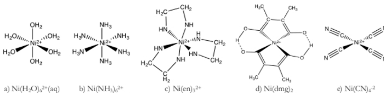
Figure 1. Structures of nickel (II) coordination complexes a-e.
