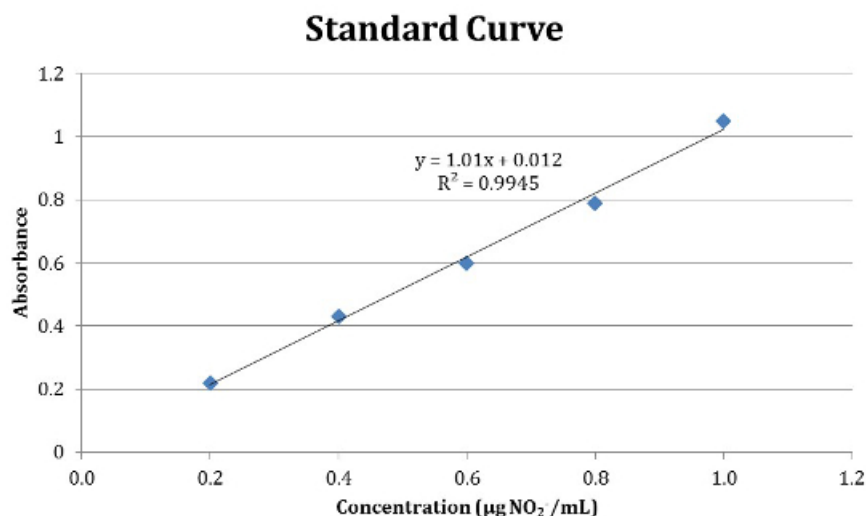
Figure 4. A standard curve plot of Absorbance vs. Concentration of NO 2 - .
