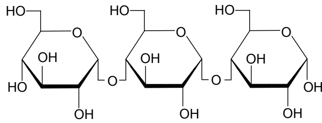
maltotriose
