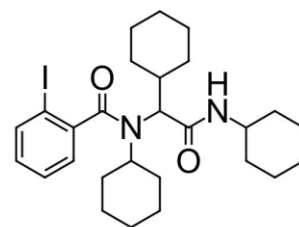
masarimycin
